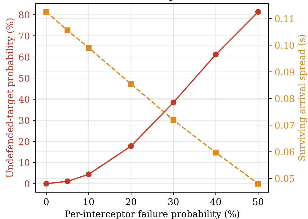
(c) Partial interceptor failure
