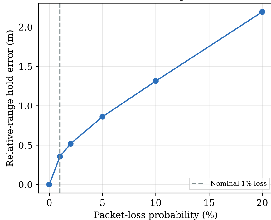
(b) Communication packet loss
