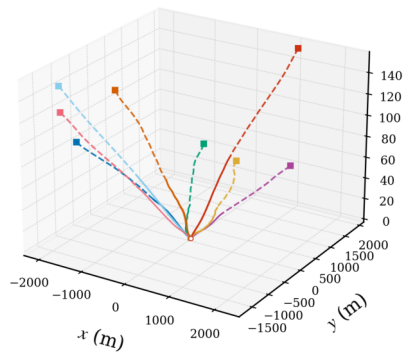
(a) 3-D engagement trajectories
