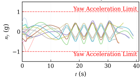
(c) Normal load n_y
