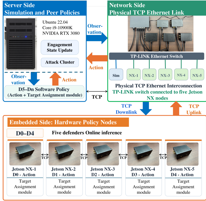
Fig. 7. HIL platform.
