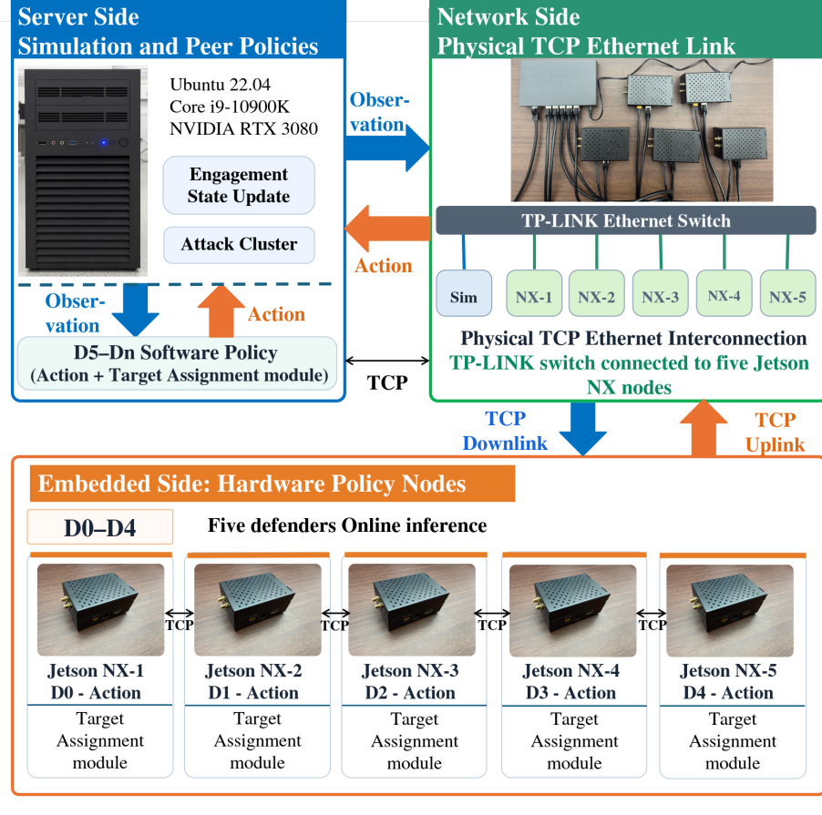
Fig. 7. HIL platform.
