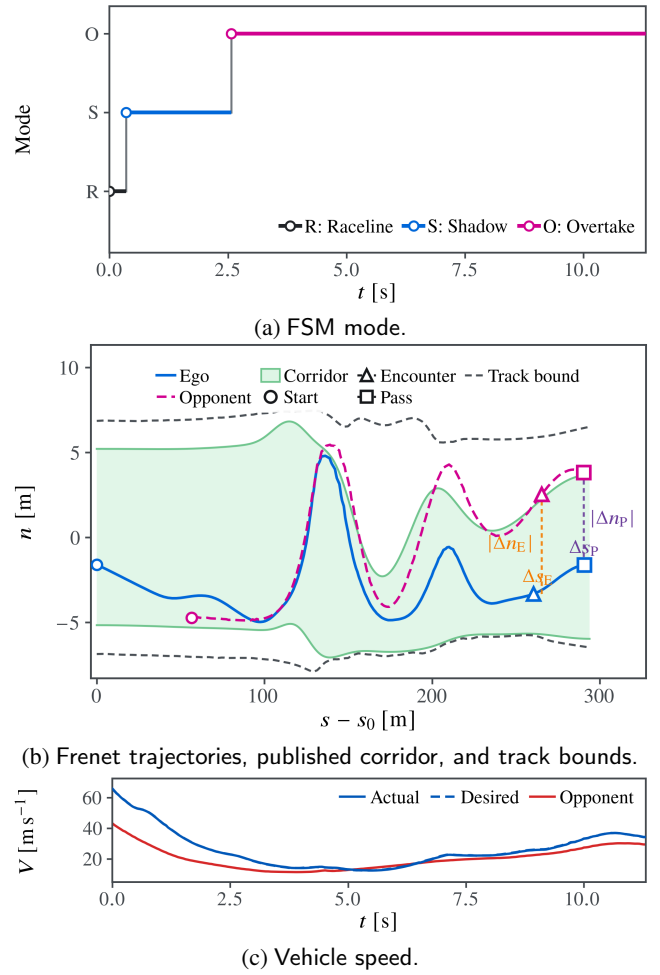
Figure 7: Tactical-mode sequence, Frenet trajectories and corridor, and speed response in Case 2.
