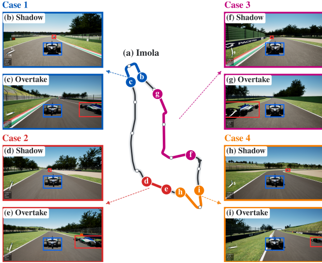
Figure 9: Representative overtaking events on the unseen Imola circuit. The central map localizes the SHADOW and OVERTAKE phases of four events, with the corresponding simulator views arranged around the map. Blue and red boxes indicate the ego and opponent vehicles, respectively.
