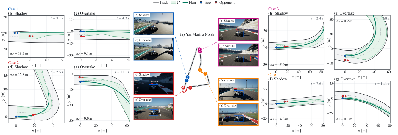
Figure 4: Representative overtaking situations on Yas Marina North.
