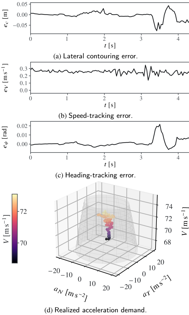
Figure 6: Closed-loop tracking errors and realized acceleration demand in Case 1.
