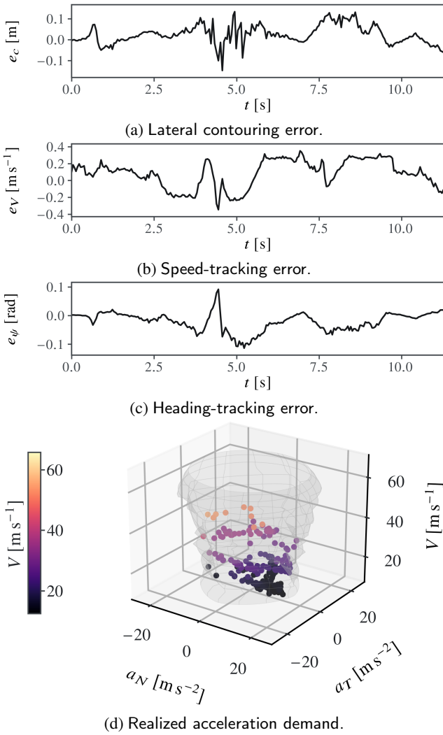
Figure 8: Closed-loop tracking errors and realized acceleration demand in Case 2.
