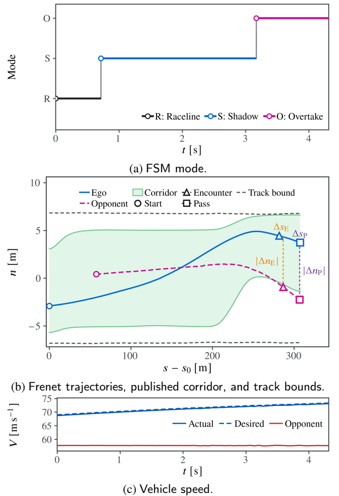
Figure 5: Tactical-mode sequence, Frenet trajectories and corridor, and speed response in Case 1.
