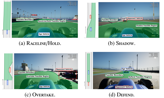
Figure 3: Geometric semantics of the persistent modes. Green regions are the published feasible corridors. SHADOW prepares the locked side, OVERTAKE excludes the opponent footprint on that side, and DEFEND reserves the blocking corridor; the common executor receives only the resulting bounds and speed cap.
