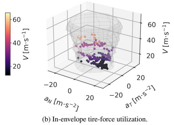
Figure 12: Scenario II clearance and tire-force diagnostics. (a) Relative separation remains outside simultaneous contact thresholds during the pass. (b) The surface and points show the 193 of 230 logged samples satisfying the displayed \rho \leq 1 envelope. The 37 out-of-envelope samples remain in the source log and are not plotted; this panel is not a hard safety certificate.
