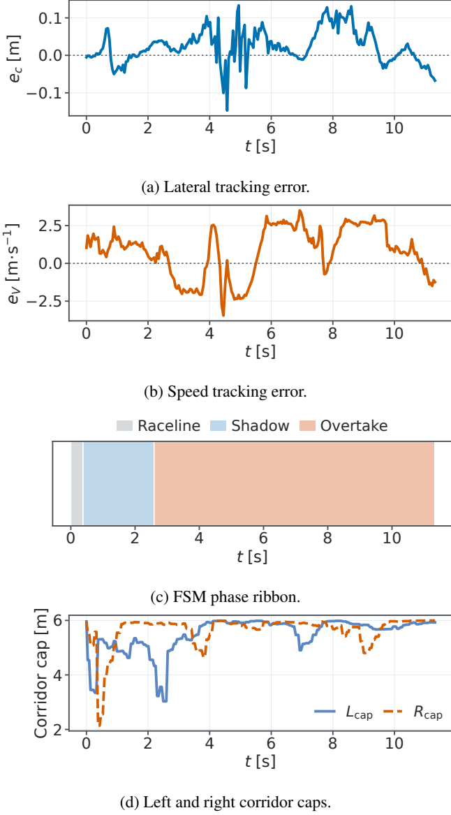
Figure 11: Scenario II tracking and tactical-state responses. (a,b) Tracking remains bounded through braking, cornering, and acceleration. (c) The raw mode sequence shows uninterrupted OVERTAKE commitment after 2.59 s. (d) The changing left and right caps expose the learned corridor adaptation that is hidden by a discrete maneuver label.
