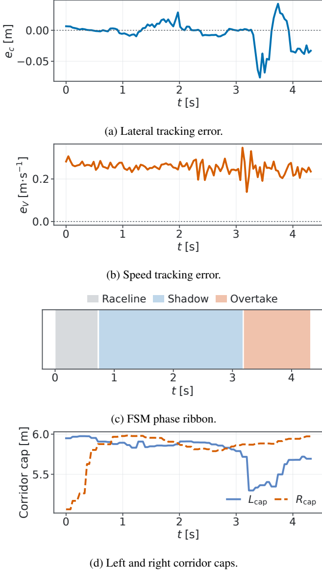
Figure 7: Scenario I tracking and tactical-state responses. (a,b) The common executor tracks the corridor-derived path and speed references. (c) The phase sequence exposes the transition from approach to committed overtake. One of 109 raw mode samples is normalized for display as described in the text. (d) The dimensional corridor caps remain non-degenerate throughout the pass.
