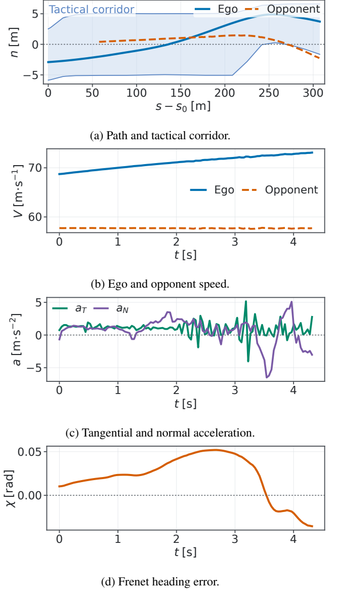
Figure 6: Scenario I closed-loop execution. (a) The ego path remains inside the causal tactical-corridor history. (b) The speed advantage closes the initial gap. (c,d) Acceleration and heading responses show how the common executor realizes the selected side. Panel (c) contains all 109 logged samples.
