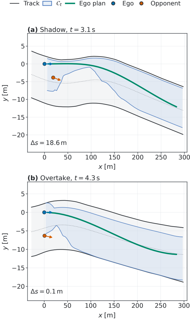
Figure 5: Scenario I interaction geometry. (a) The pre-pass plan is formed inside the game-layer corridor while the vehicles remain separated by \Delta s = 18.6 m. (b) The selected side and corridor persist to the order crossover. Blue denotes C_t , green the finite-horizon ego plan, and the arrows vehicle headings.
