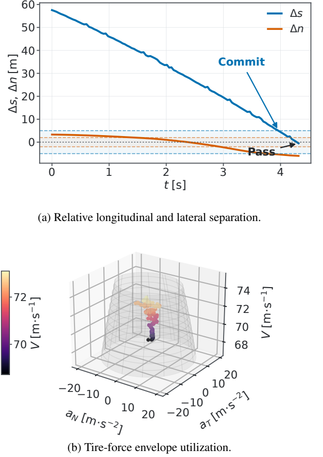
Figure 8: Scenario I supporting clearance and physical-admissibility checks. (a) The shaded threshold bands show the rectangular contact test; Commit and Pass mark the final +5-m crossing and the first negative \Delta s sample. (b) All 109 logged acceleration samples are shown relative to the speed-dependent tire-force envelope.
