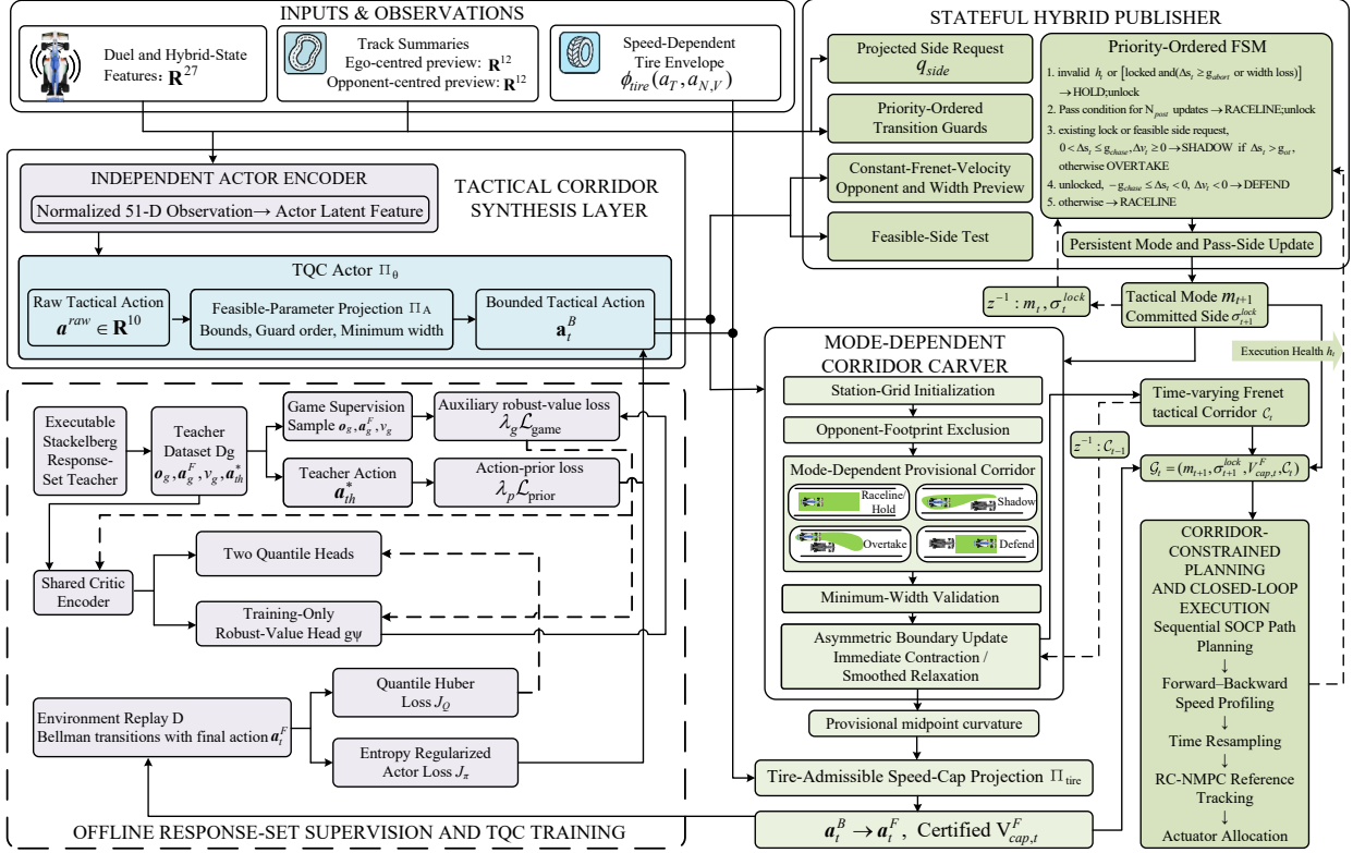
Fig. 2 Overview of the proposed game-supervised tactical feasible-region framework.
