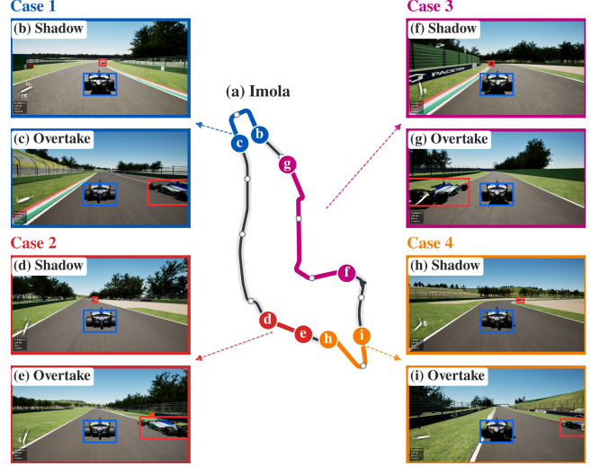
Fig. 10 Representative overtaking events on the unseen Imola circuit. The central map localizes the SHADOW and OVERTAKE phases of four events, with the corresponding simulator views arranged around the map. Blue and red boxes indicate the ego and opponent vehicles.
