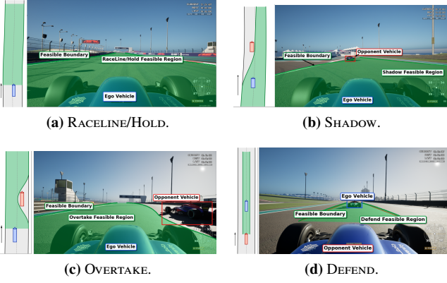
Fig. 2 Nominal geometry of the persistent tactical modes. Each panel pairs the Frenet feasible region with the corresponding simulator view; the shaded interval is the region delivered to the planner.
