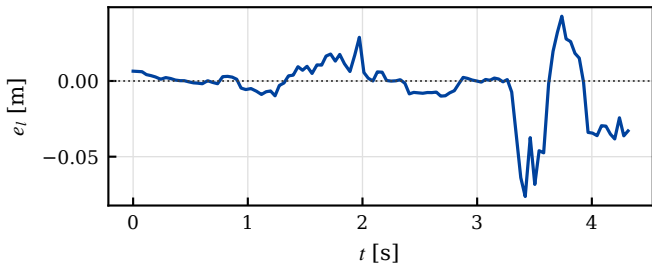
(a) Lateral tracking error
