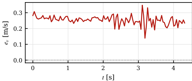
(b) Speed tracking error
