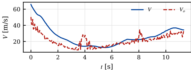
(a) Speed profile
