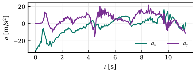
(b) Longitudinal and lateral acceleration
