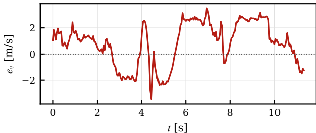
(b) Speed tracking error
