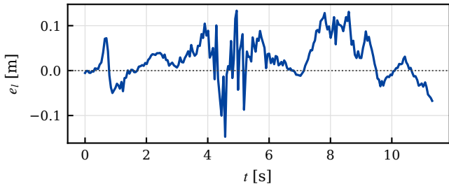
(a) Lateral tracking error
