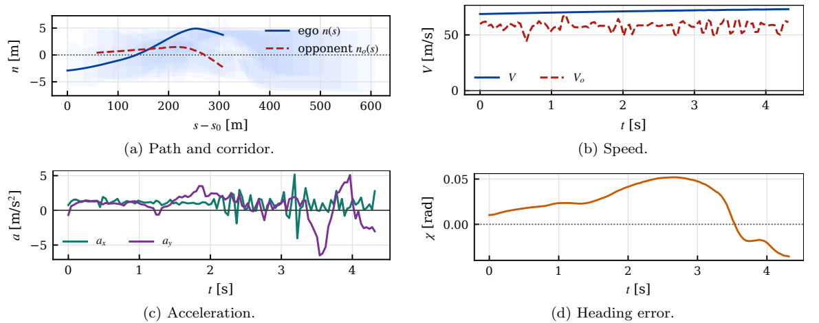
Figure 5: Scenario I closed-loop execution states.
