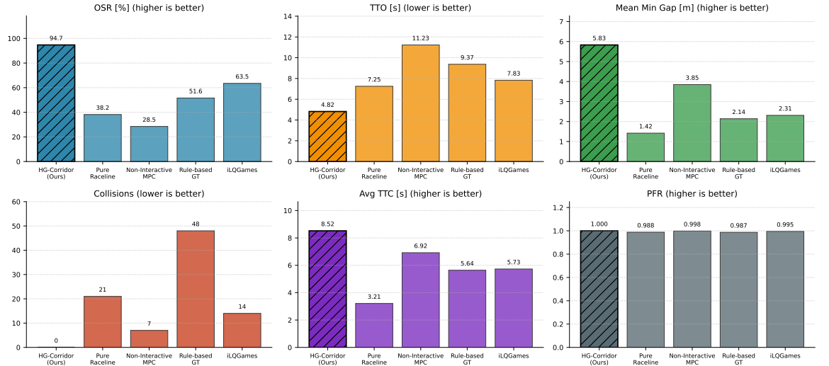
Figure 17: Aggregate comparison of key safety and performance metrics across methods using the values reported in Table 2. Hatched bars mark the best method for each metric.
