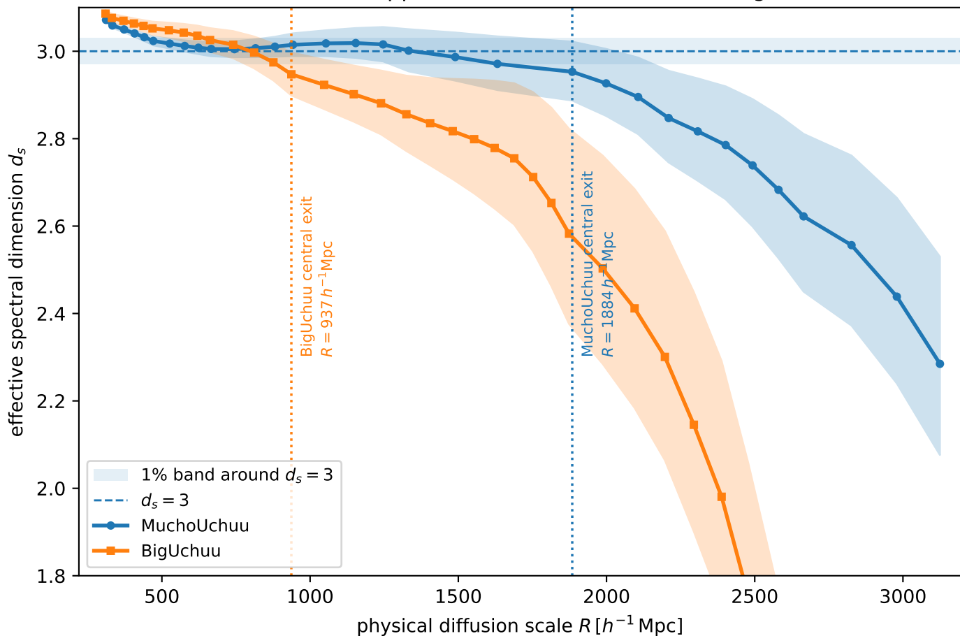
Finite-volume suppression in MuchoUchuu and BigUchuu
