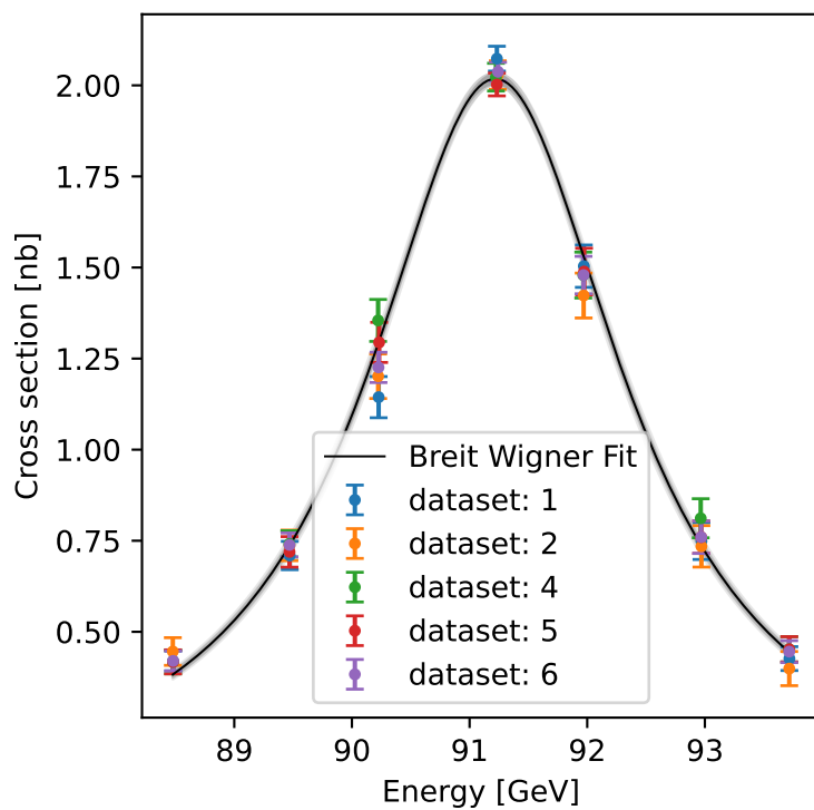
\tau^+\tau^- channel
