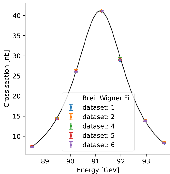
\bar{q}q channel
