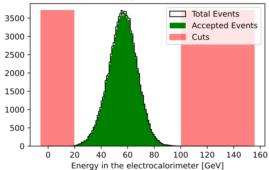
\bar{q}q channel
