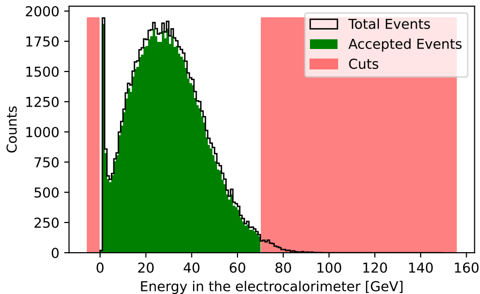
\tau^+\tau^- channel
