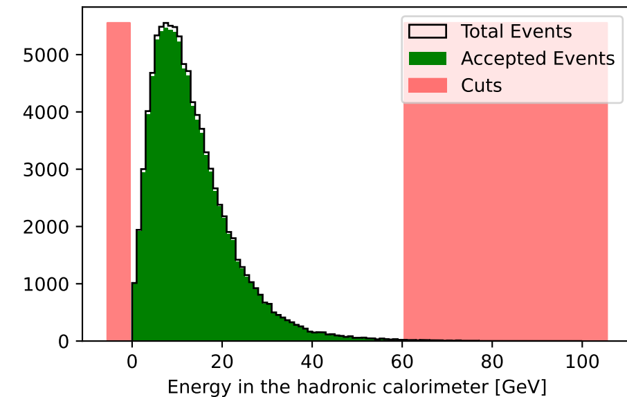
\bar{q}q channel
