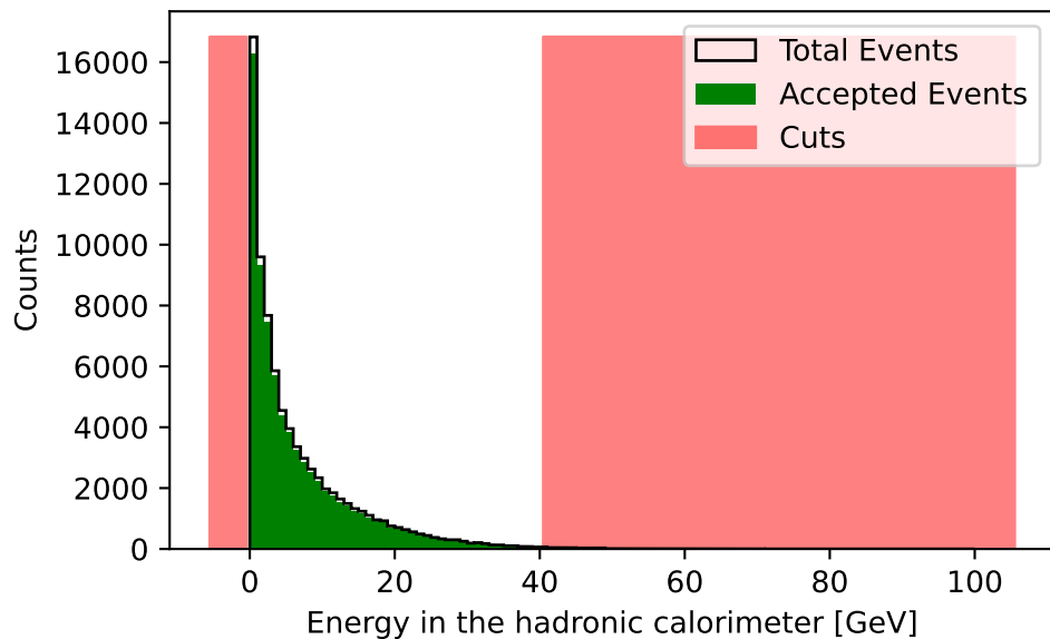
\tau^+\tau^- channel
