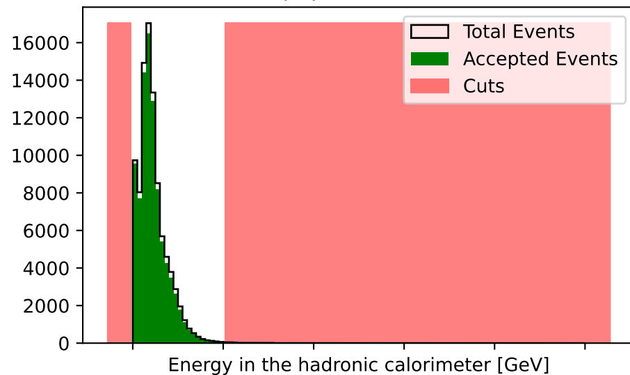
\bar{q}q channel
