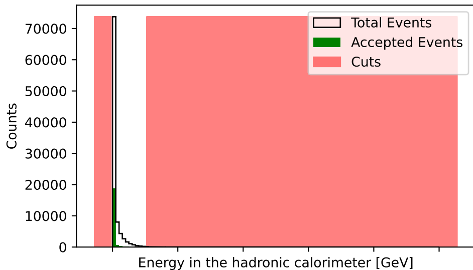
\tau^+\tau^- channel
