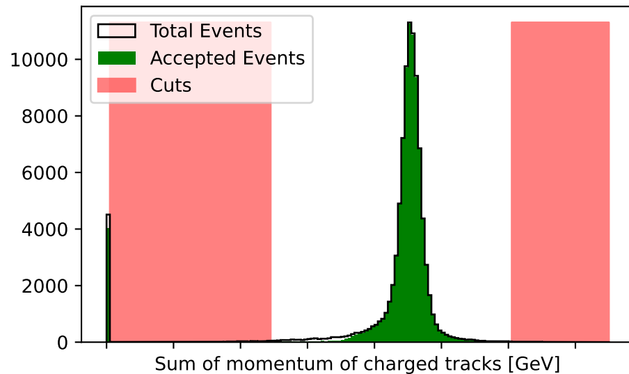
\bar{q}q channel
