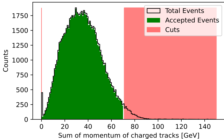
\tau^+\tau^- channel
