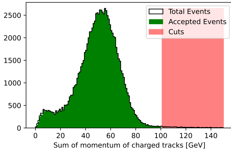
\bar{q}q channel
