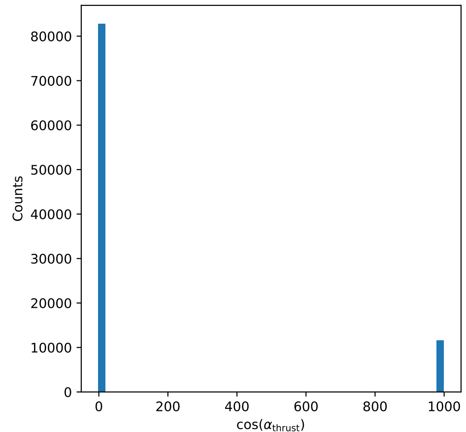
m^+m^- channel
