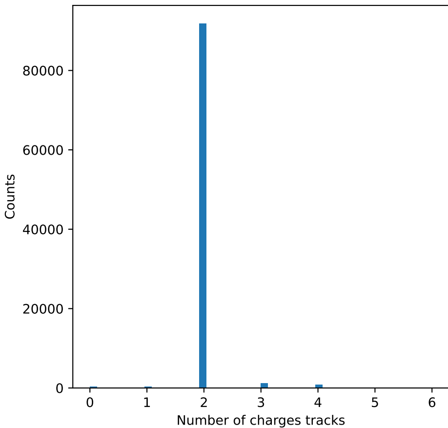
m^+m^- channel
