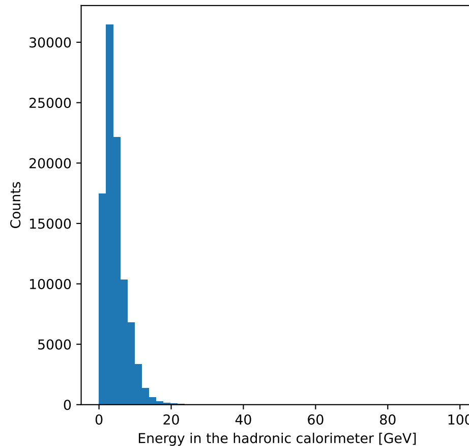
m^+m^- channel
