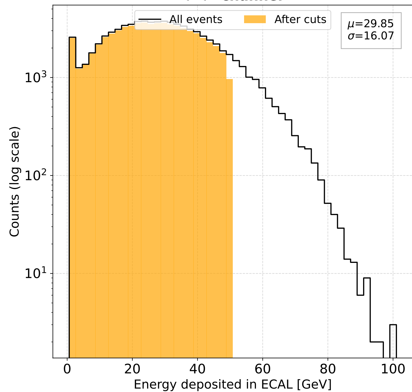
\tau^+\tau^- channel
