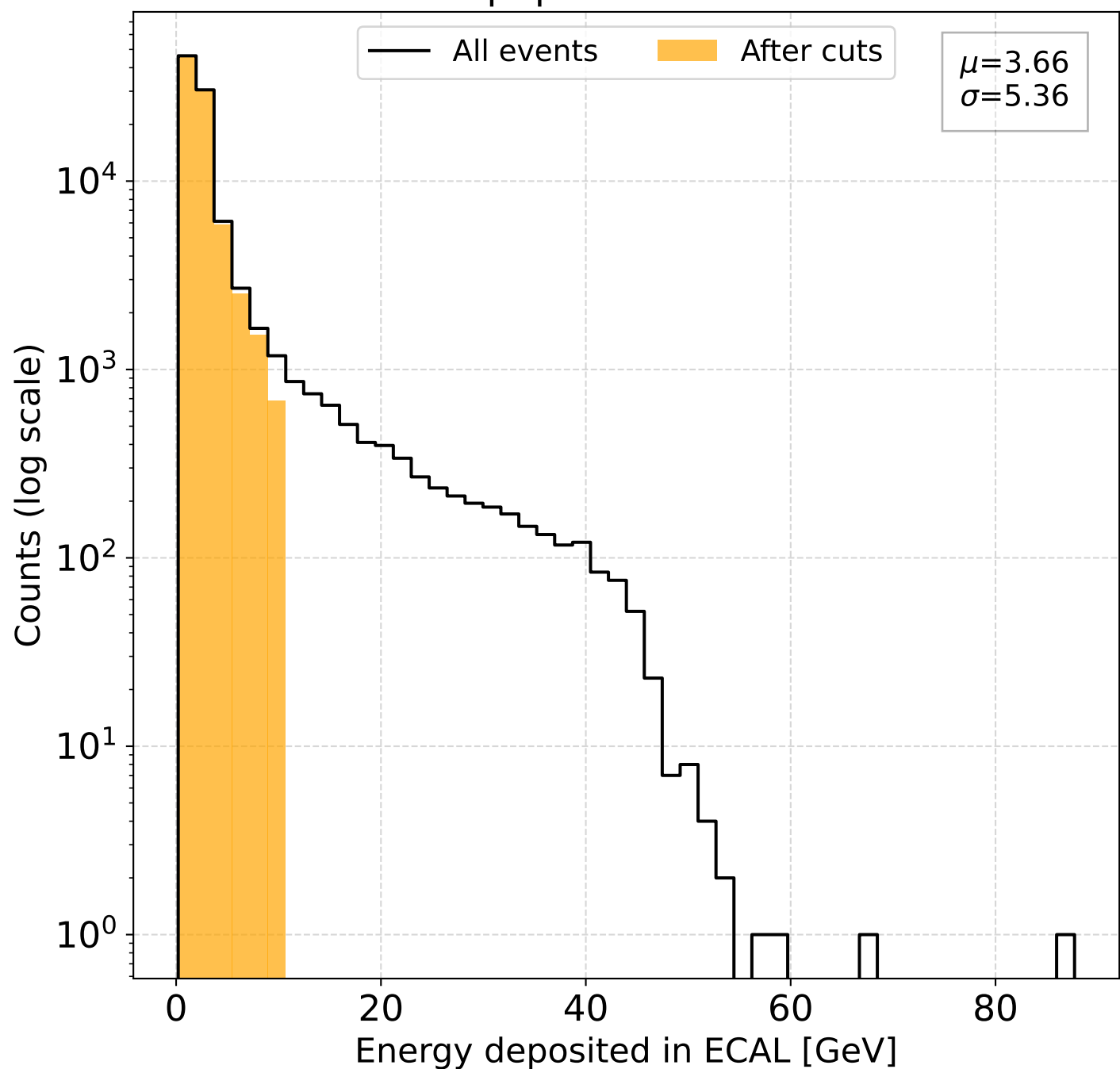
q^+q^- channel
