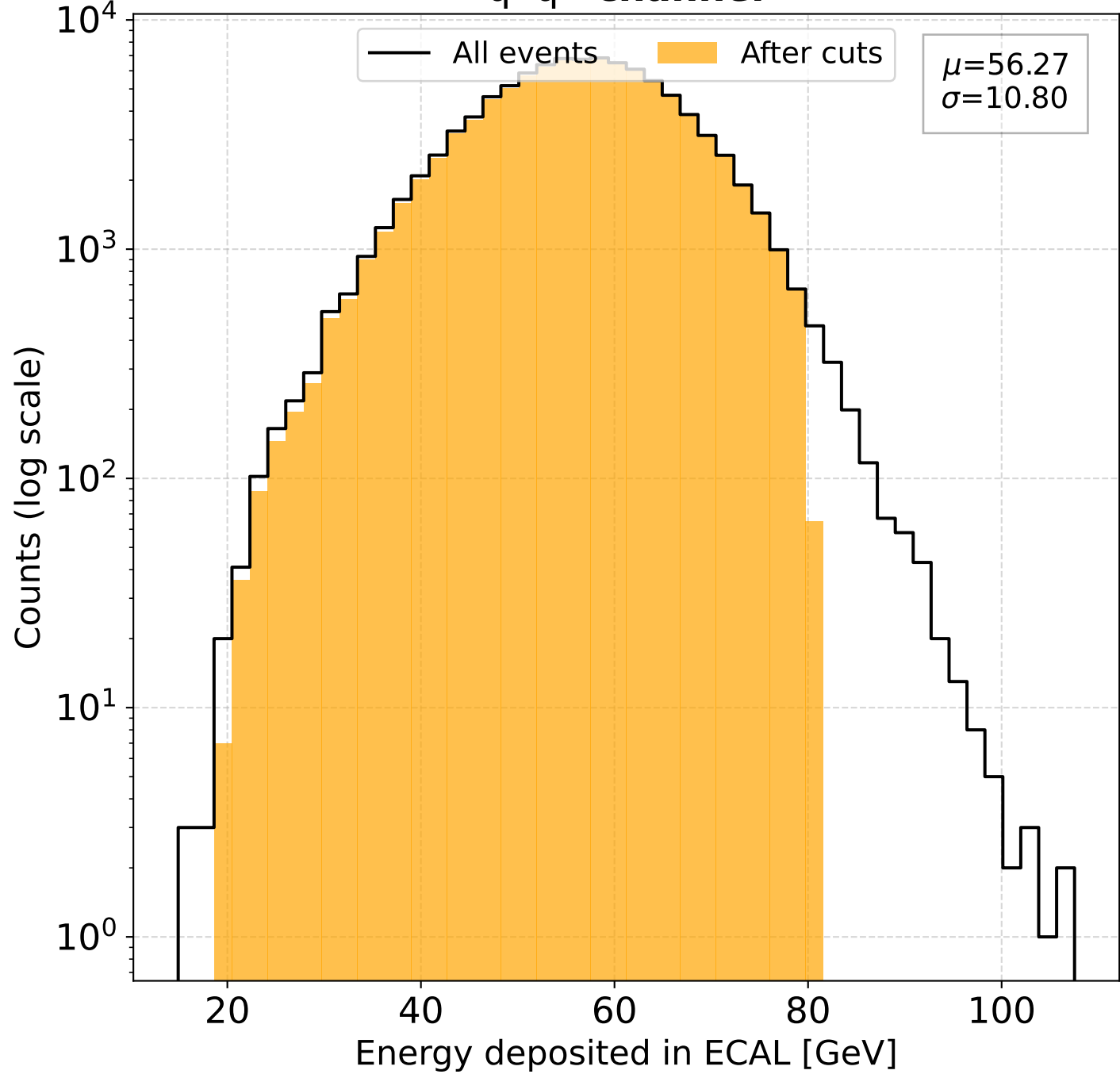
q^+q^- channel
