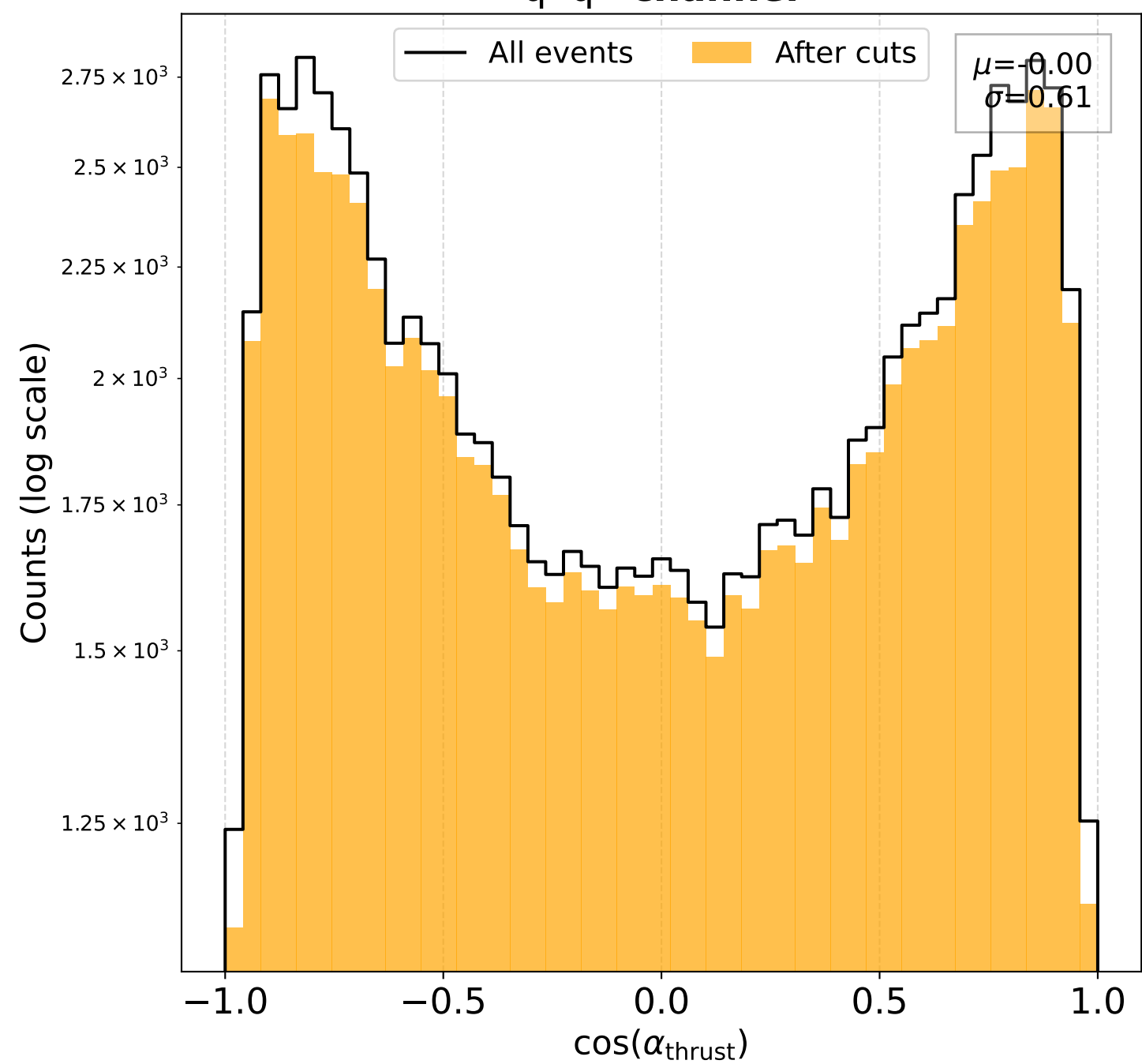
q^+q^- channel
