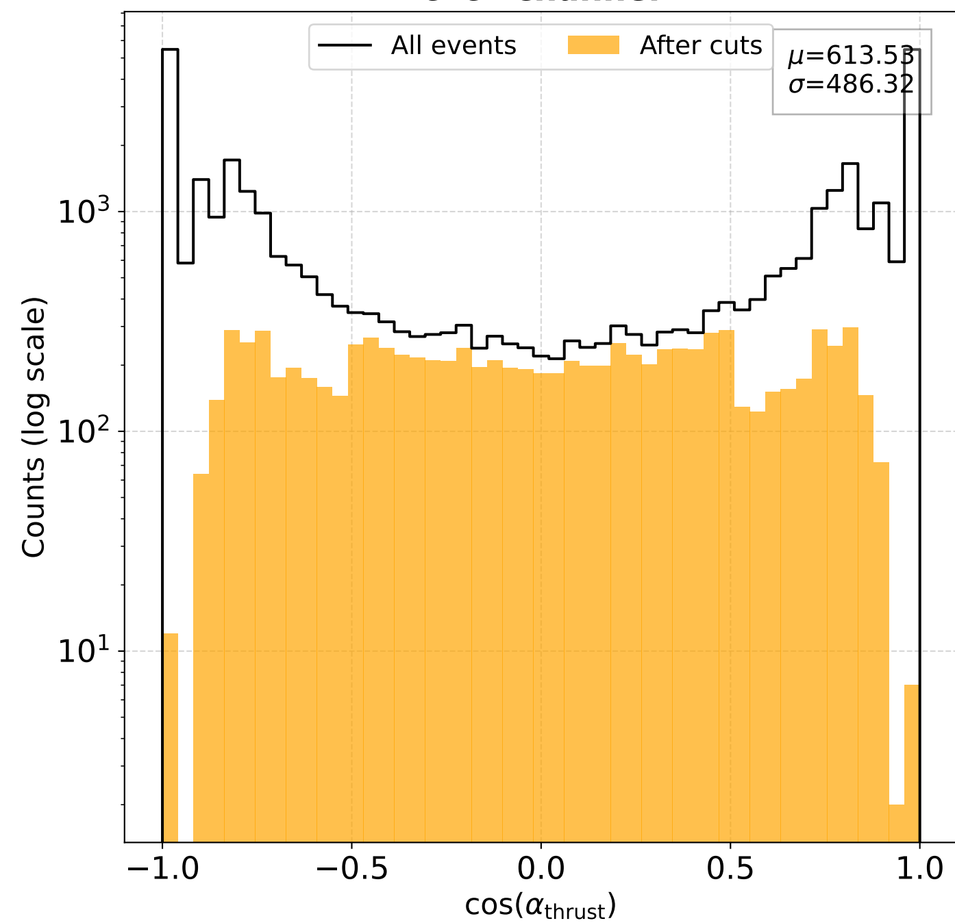
\tau^+\tau^- channel
