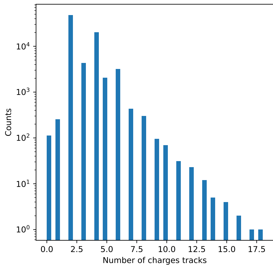
\tau^+\tau^- channel
