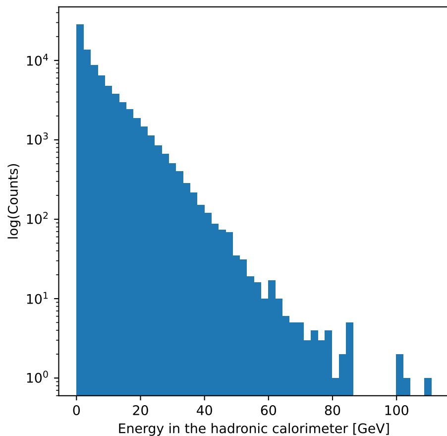
\tau^+\tau^- channel
