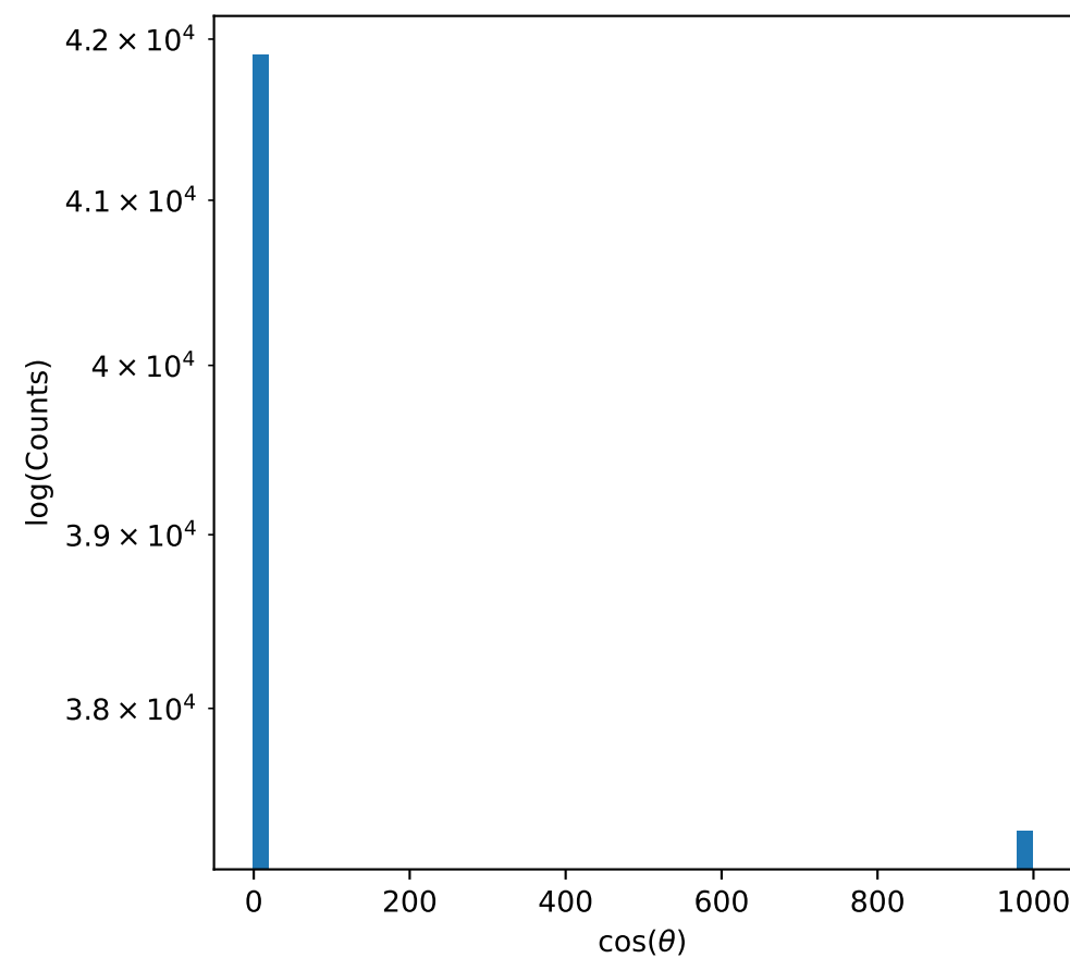
\tau^+\tau^- channel
