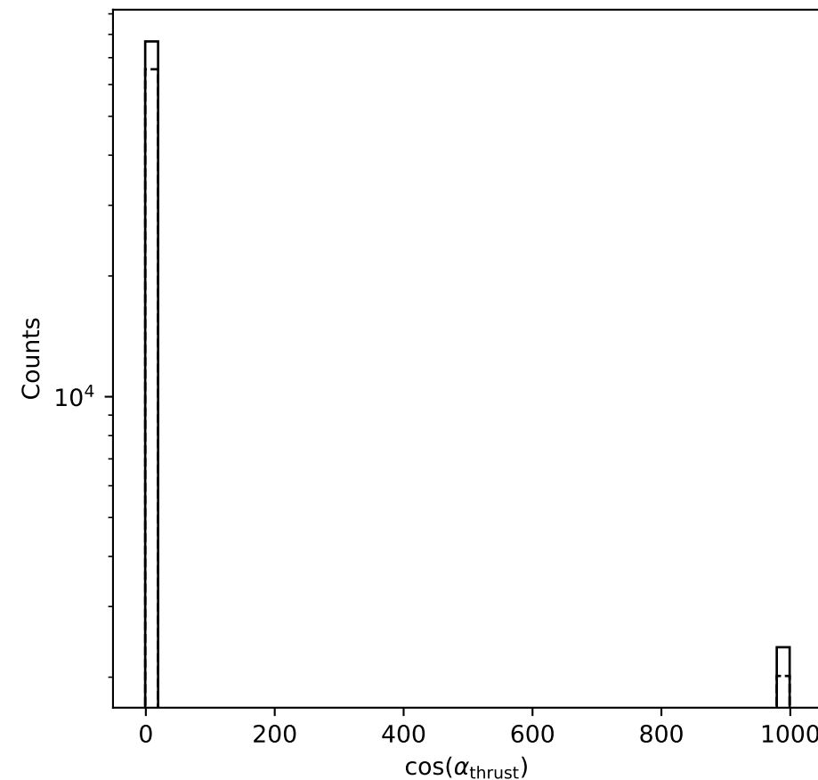
\tau^+\tau^- channel
