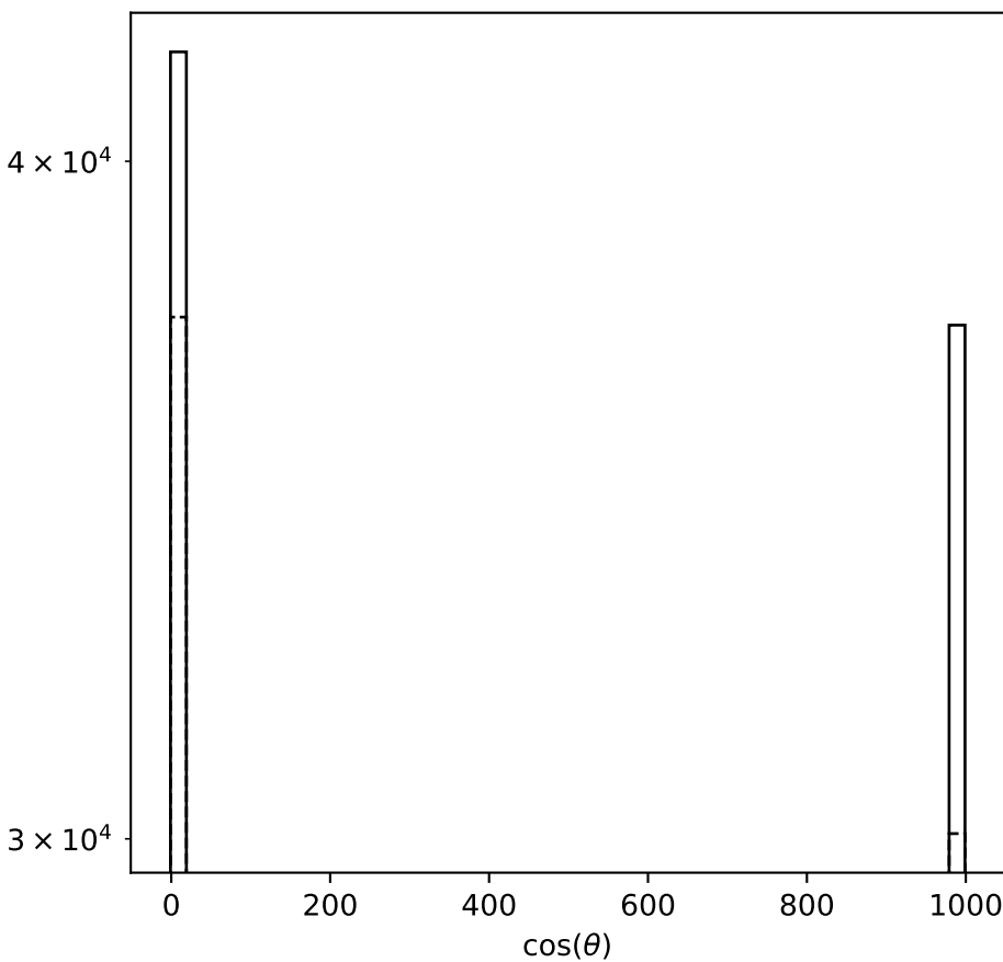
\tau^+\tau^- channel
