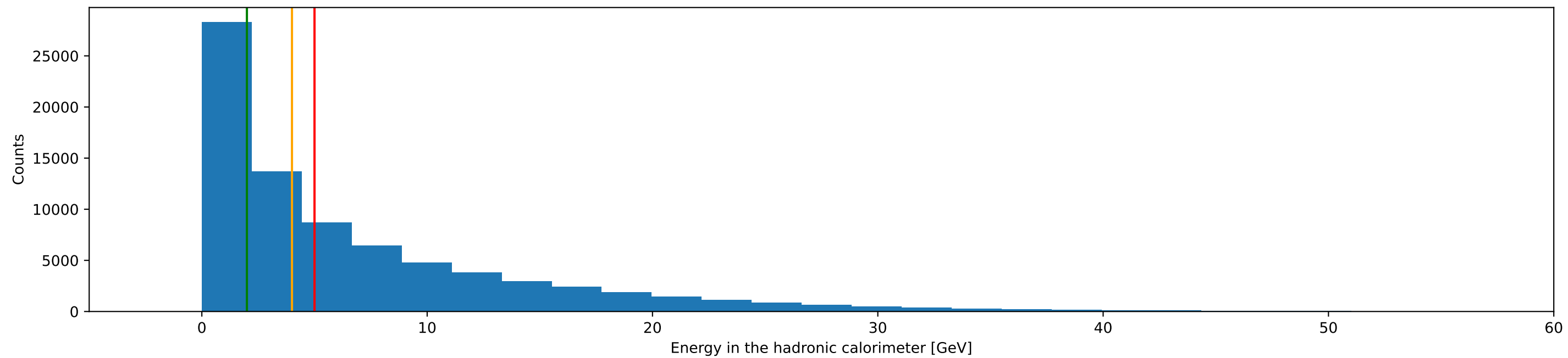
q^+q^- channel
