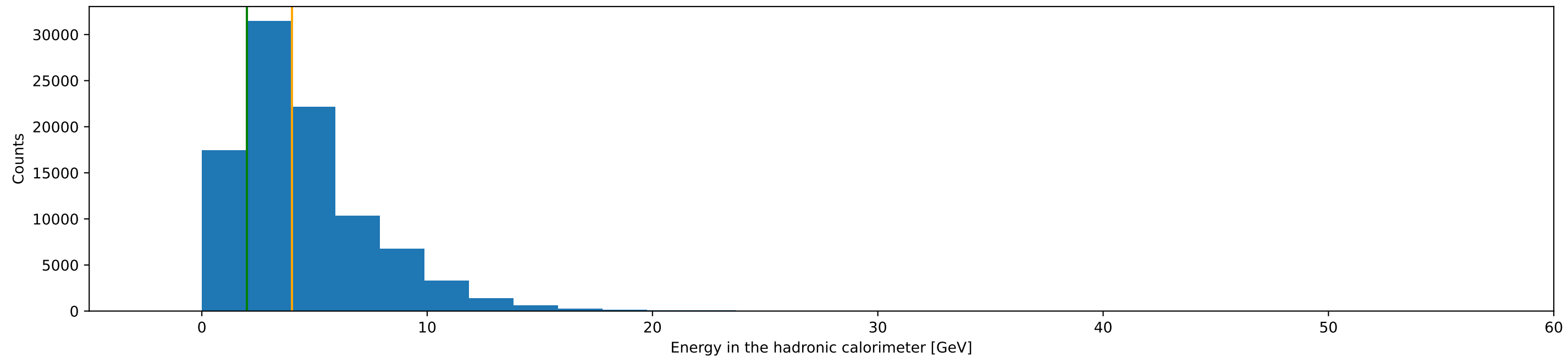
t^+t^- channel
