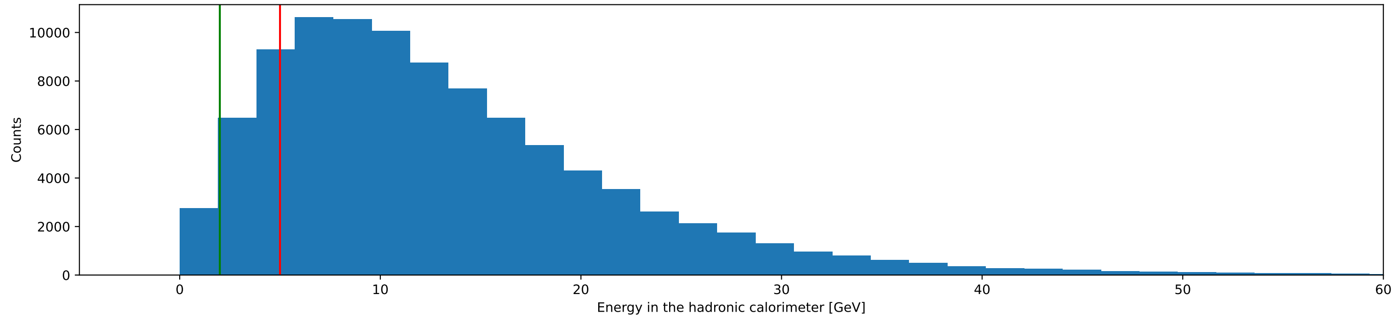
q^+q^- channel
