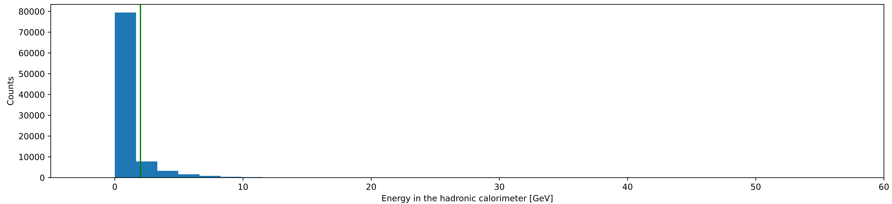
m^+m^- channel
