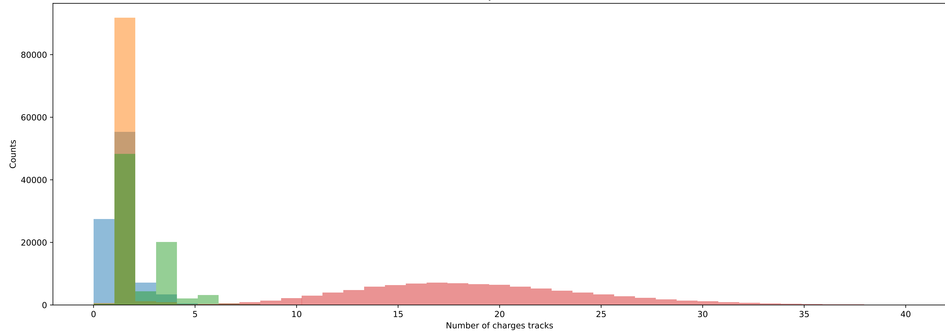
Decay channel
