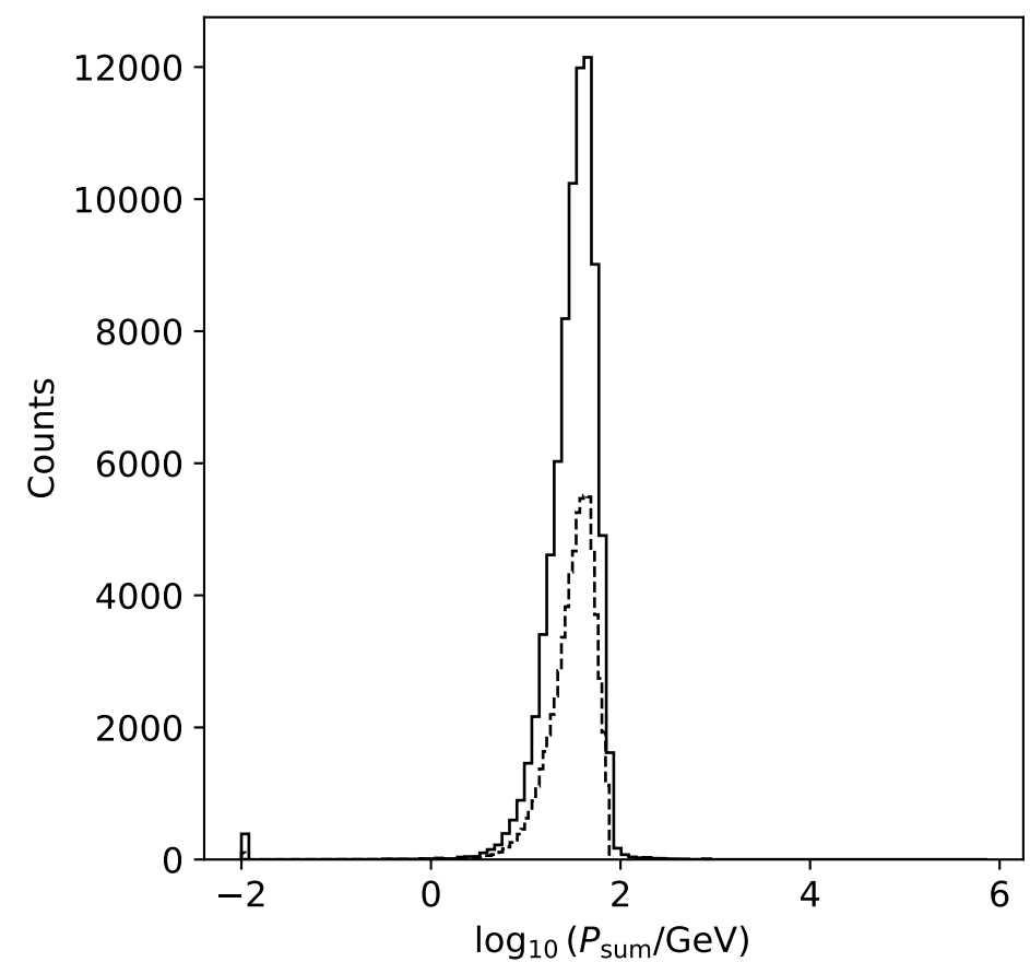
\tau^+\tau^- channel
