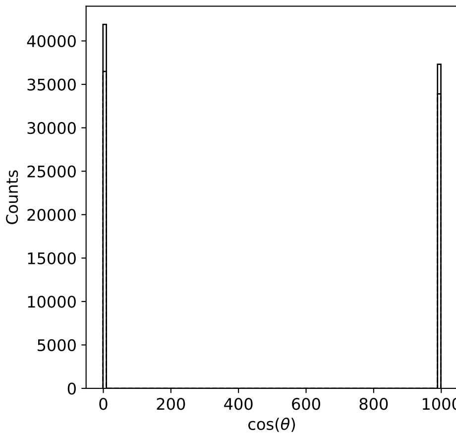
\tau^+\tau^- channel
