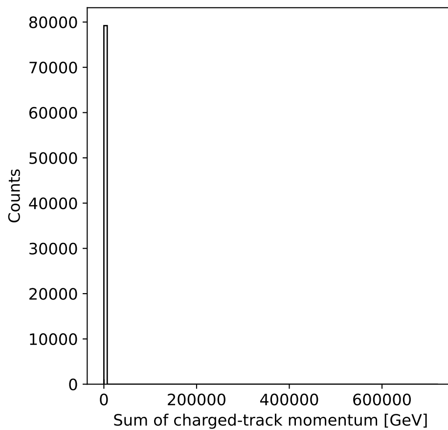
\tau^+\tau^- channel
