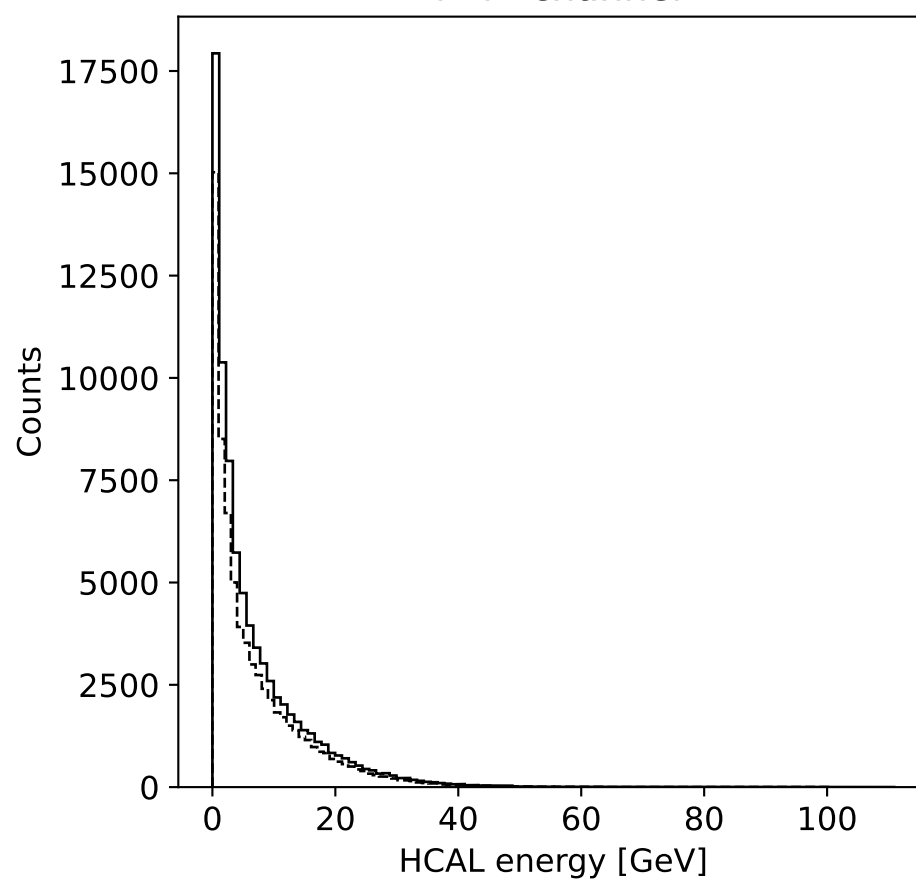
\tau^+\tau^- channel
