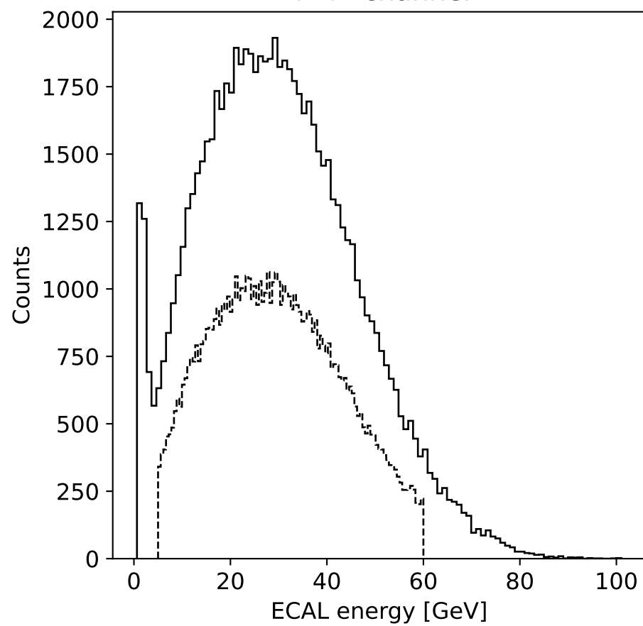
\tau^+\tau^- channel
