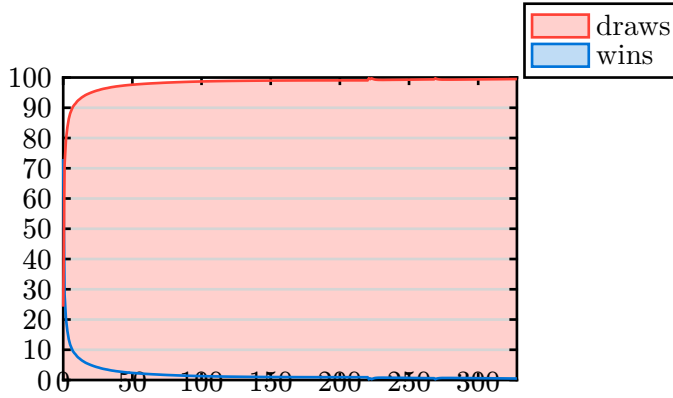
Pseudo Unmasked
