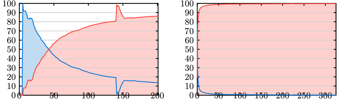
Pseudo Unmasked
