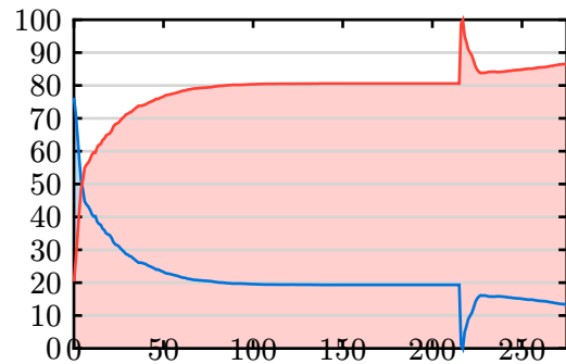
Pseudo Masked
