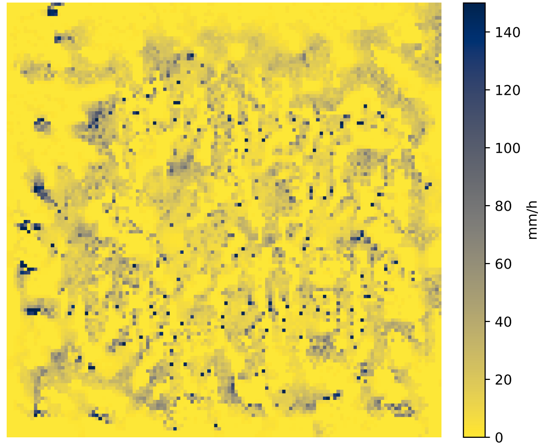
Dreamt (Constrained)
