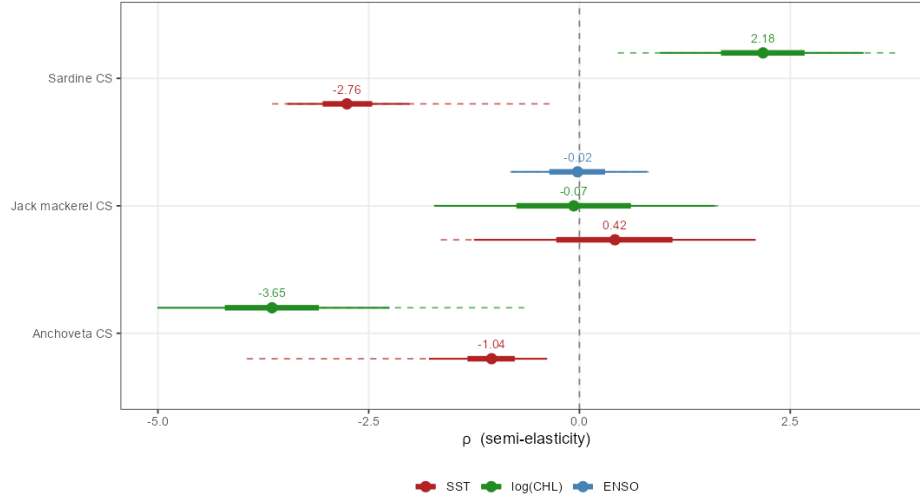
Figure 3: Posterior and prior distributions of the climate shifters \rho_s^{SST} , \rho_s^{CHL} , and \rho_s^{ENSO} by stock. Solid lines show the posterior 90% (thin) and 50% (thick) credible intervals; dashed lines show the prior 90% credible interval. Anchoveta and sardine show substantial posterior updating with narrow credible intervals excluding zero. Jack mackerel posteriors (SST, CHL, ENSO) coincide with their vague priors centred at zero, indicating non-identification.
