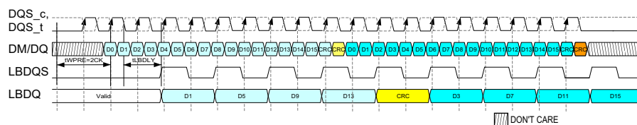
Figure 176 — Loopback Write Burst with CRC Output Mode 4-Way PhaseB with CRC, No Gap Example
