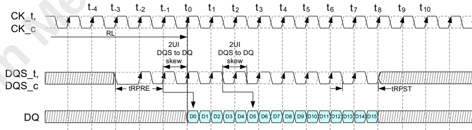
Figure 244 — Read Burst Example for Pin DQx Depicting Bit 0 and 5 Relative to the DQS Edge for 2 UI Skew with Read DQS Offset Timing Set to 1 Clock (2UI)
