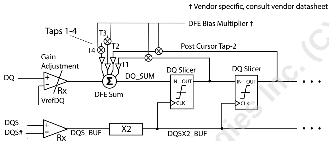
Figure 143 — 4-Tap DFE Example
