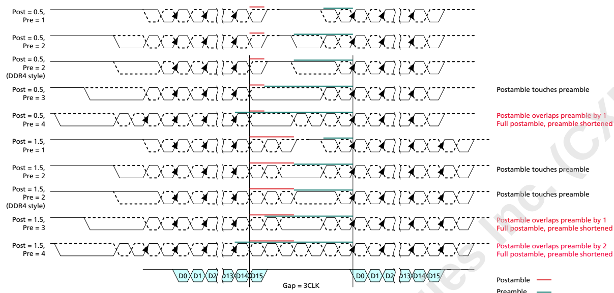
Figure 21 — Example of Consecutive Reads Operation: t_{CCD} = \text{Min} + 3
