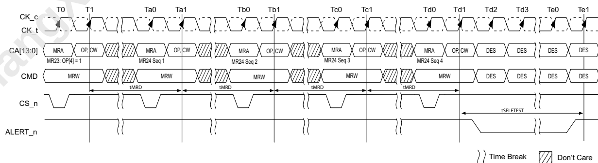
Figure 138 — MBIST Procedure
