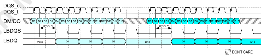
Figure 167 — Loopback Normal Output Mode 4-Way PhaseB 2CK Gap Example
