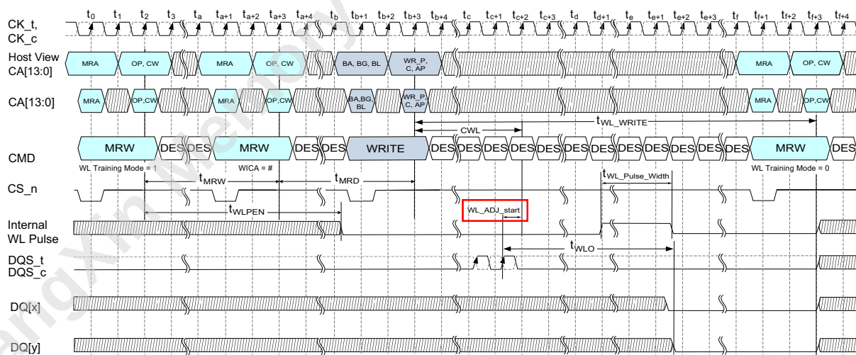
Figure 105 — Write Leveling Training Mode Timing Diagram (Internal Cycle Alignment, 2N Mode, 0 Sample)
