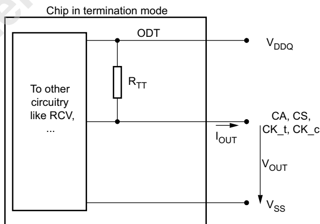
Figure 201 — A Functional Representation of the On-die Termination
