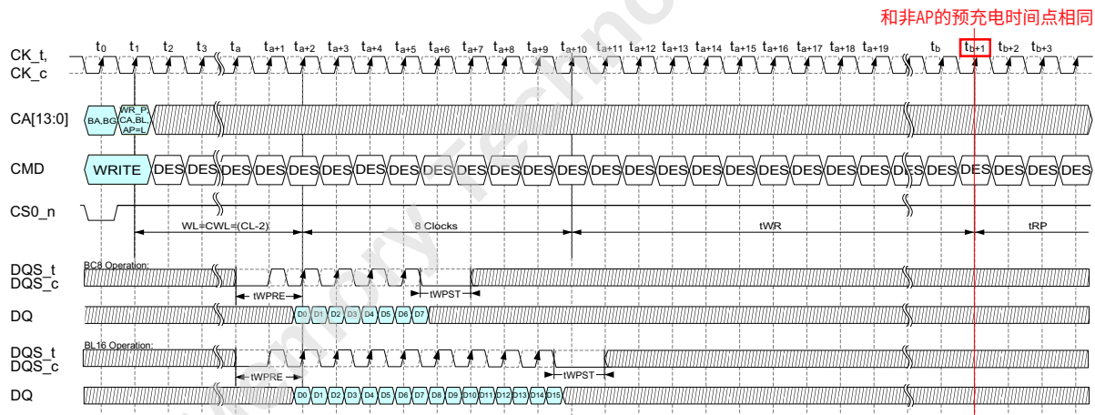
Figure 46 — WRITE (BL16) to PRECHARGE Operation with 2t_{CK} Preamble
