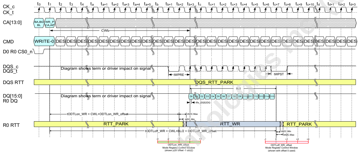
Figure 188 — Example 1 of Burst Write Operation ODT Latencies and Control Diagrams
