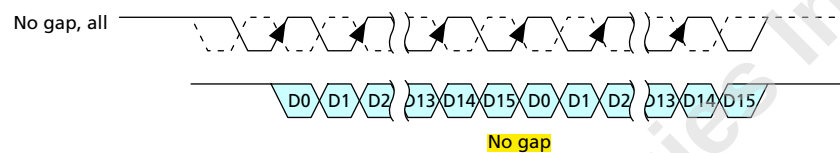
Figure 18 — Example of Seamless Reads Operation: tCCD=Min
