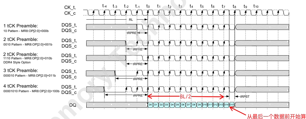
Figure 11 — Example of Read Preamble Modes (Default) with 0.5 tCK Postamble
