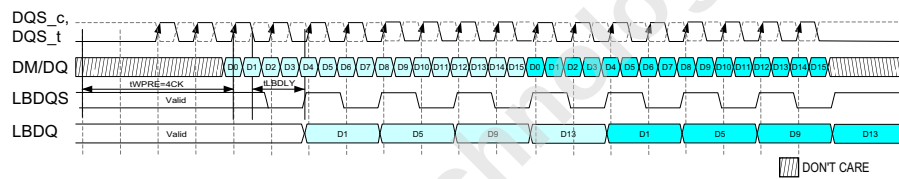
Figure 174 — Loopback Write Burst Output Mode 4-Way PhaseB Data Burst Bit and PhaseD Strobe Alignment WPRE=4CK Optional Example
