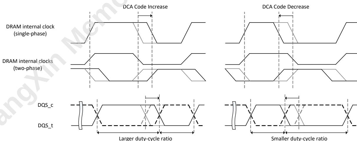
Figure 178 — Relationship Between DCA Code Change and the Single/Two-phase Internal Clock(s)/DQS Waveform (Example)
