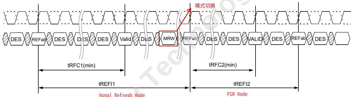
Figure 66 — Refresh Mode Change Command Timing
