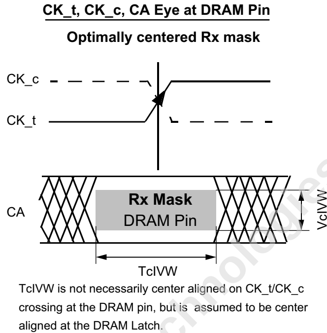
Figure 213 — CA Timings at the DRAM Pins
