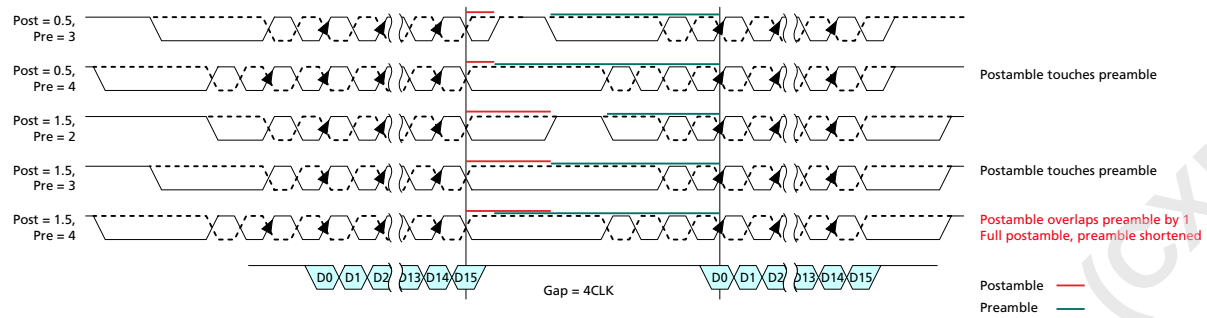
Figure 28 — Example of Consecutive Writes Operation: t_{CCD} = \text{Min} + 4
