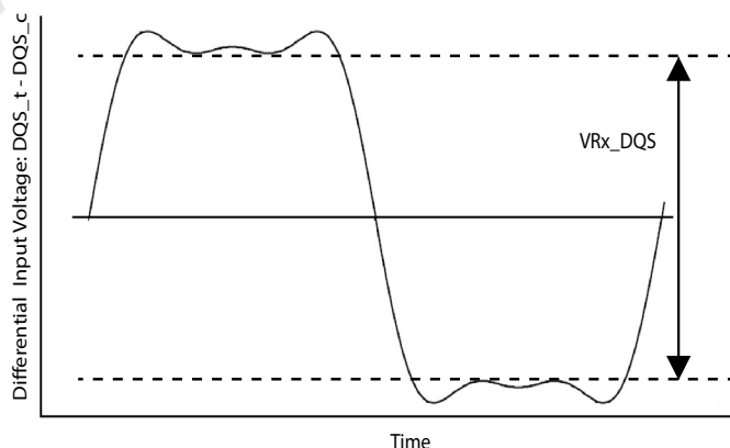
Figure 223 — VR x _DQS
