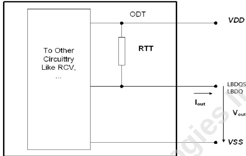
Figure 202 — Functional Representation of Loopback ODT
