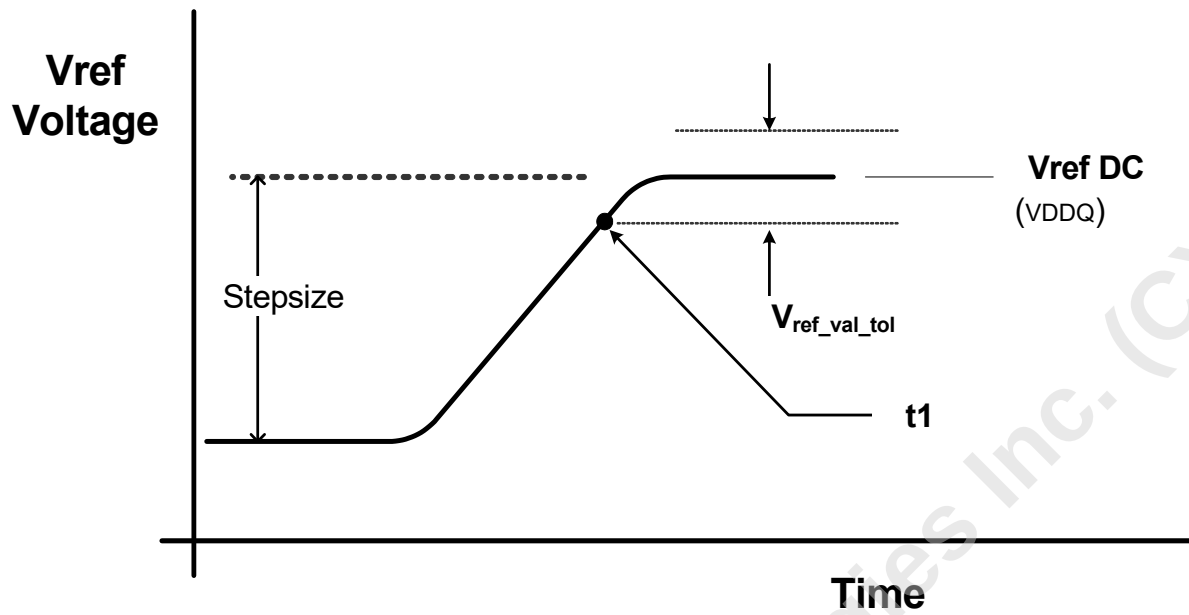
Figure 131 — VrefDQ Step Single Stepsize Increment Case
