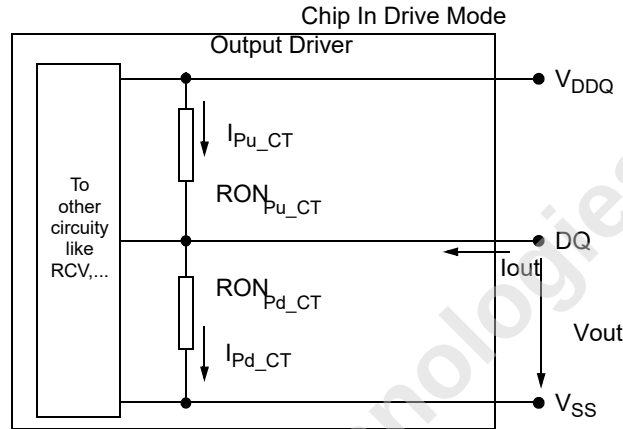
Figure 237 — Output Driver
