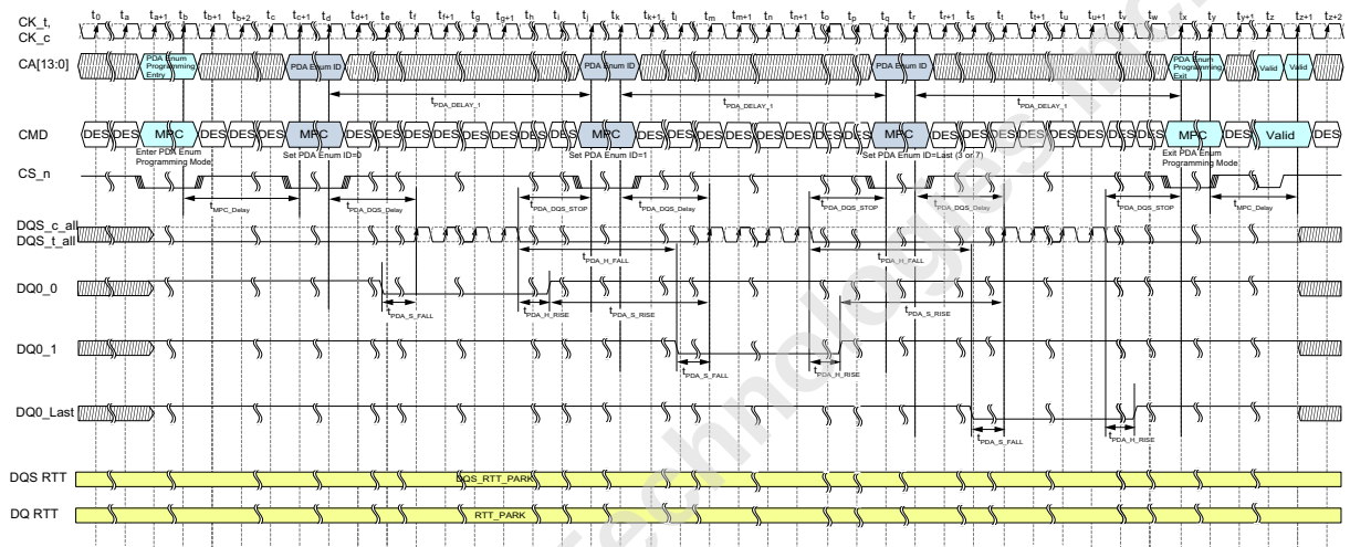
Figure 79 — Multi-Device PDA Enumerate Programming in Legacy Mode with all DQs
