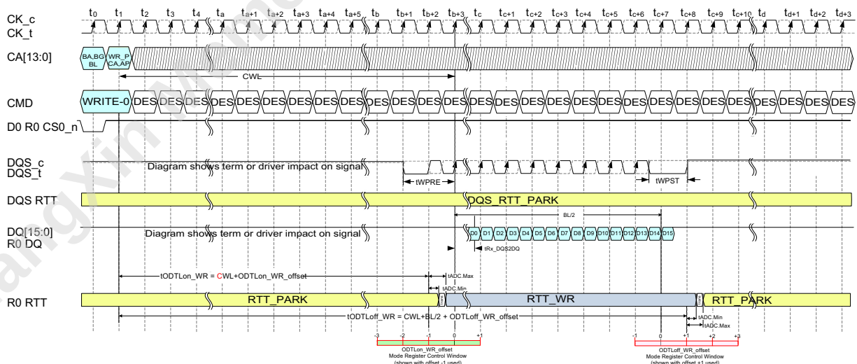
Figure 189 — Example 2 of Burst Write Operation ODT Latencies and Control Diagrams
