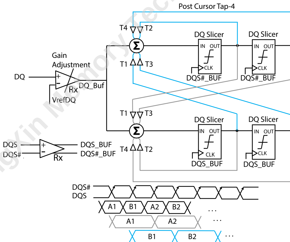
Figure 146 — 2-Way Interleave 4-Tap DFE Example
