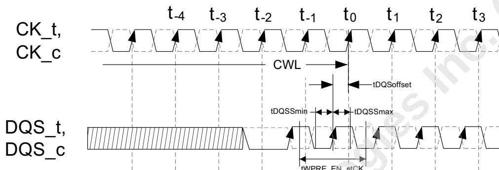
Figure 55 — t_{DQSS} : DRAM External CLK-to-DQS Variation
