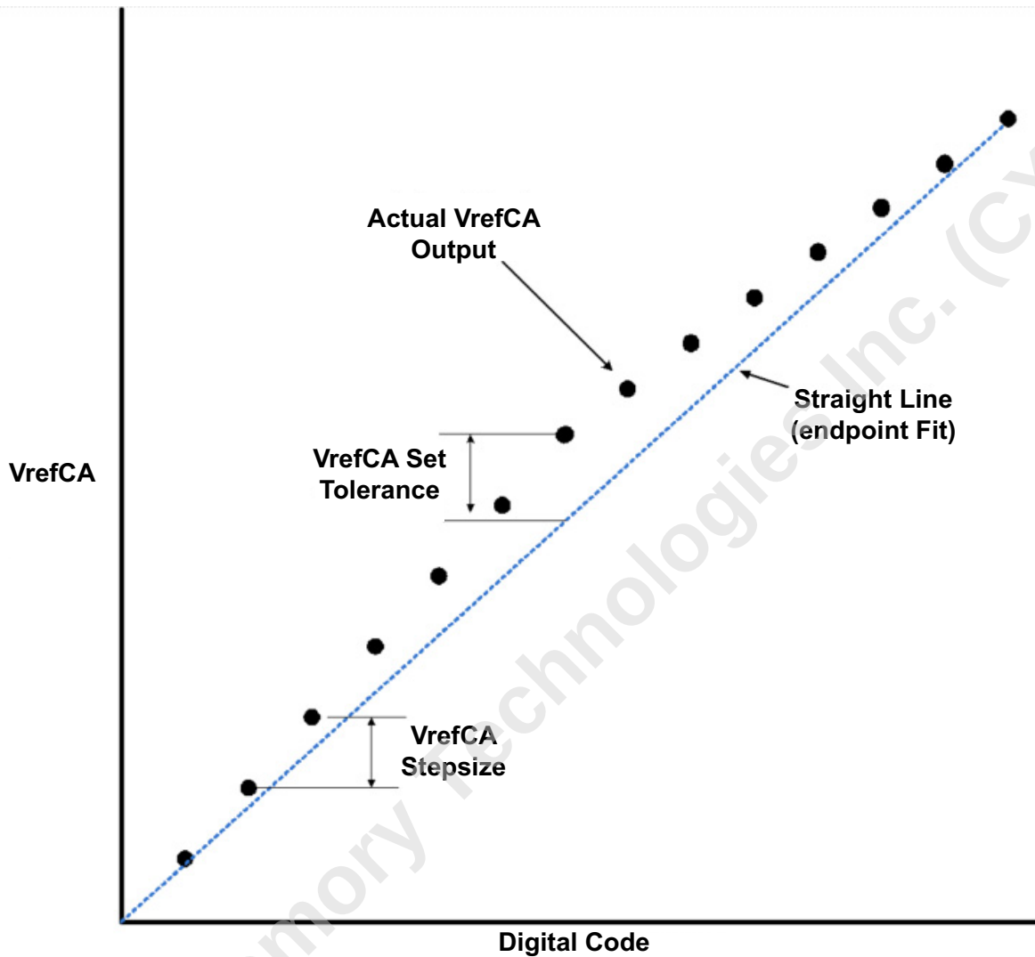
Figure 115 — Example of Vref Set Tolerance (Only Max Case is Shown) and Stepsize
