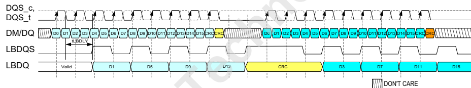
Figure 171 — Loopback Normal Output Mode 4-Way PhaseB with CRC, 2 CK Gap Example
