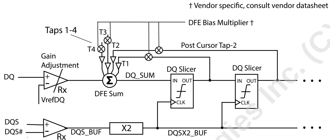
Figure 145 — 1-Way Interleave 4-Tap DFE Example
