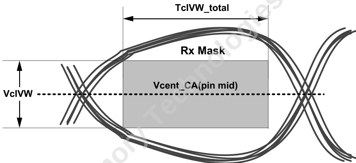
Figure 211 — CA Receiver (Rx) Mask
