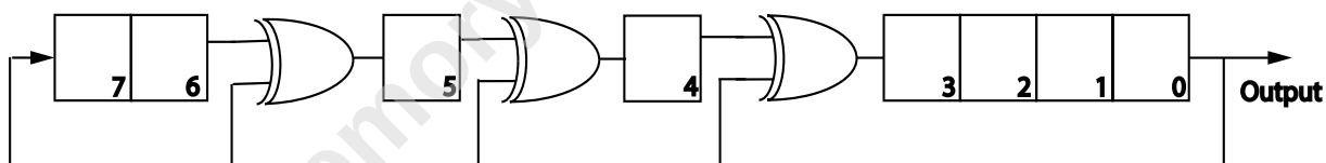
Figure 90 — Read Training Pattern LFSR
