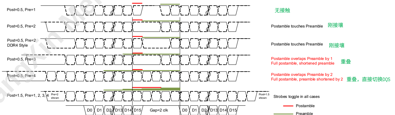
Figure 20 — Example of Consecutive Reads Operation: tCCD=Min+2
