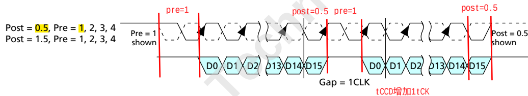
Figure 19 — Example of Consecutive Reads Operation: tCCD=Min+1
