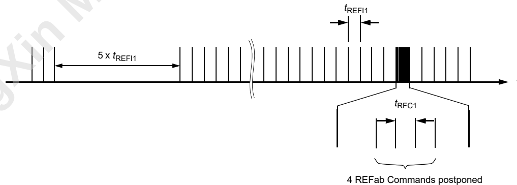
Figure 69 — Postponing Refresh Commands (Example of Normal Refresh Mode - tREFI1, tRFC1)
