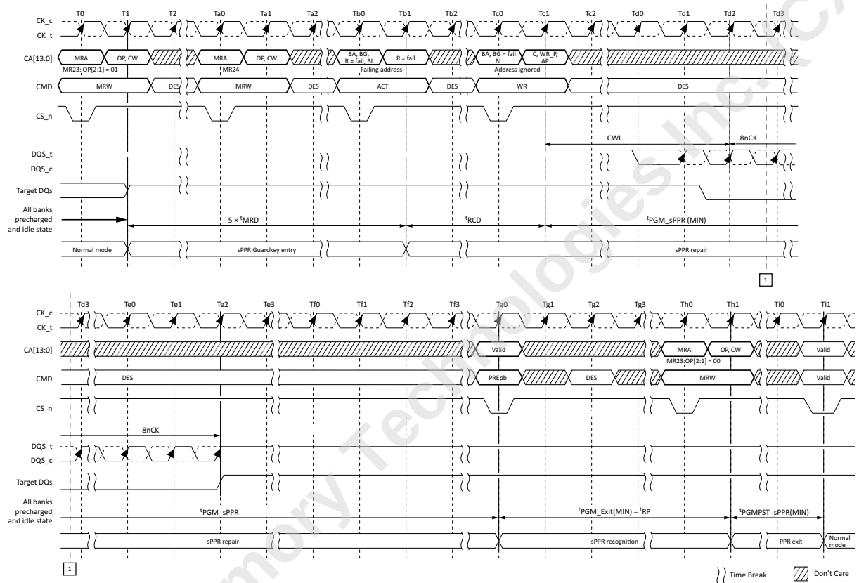
Figure 137 — sPPR Fail Row Repair
