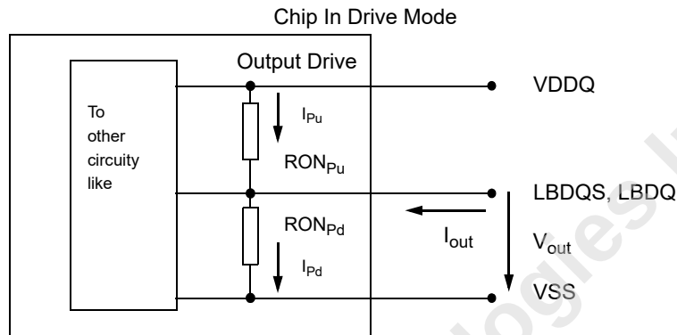
Figure 234 — Output Driver for Loopback Signals
