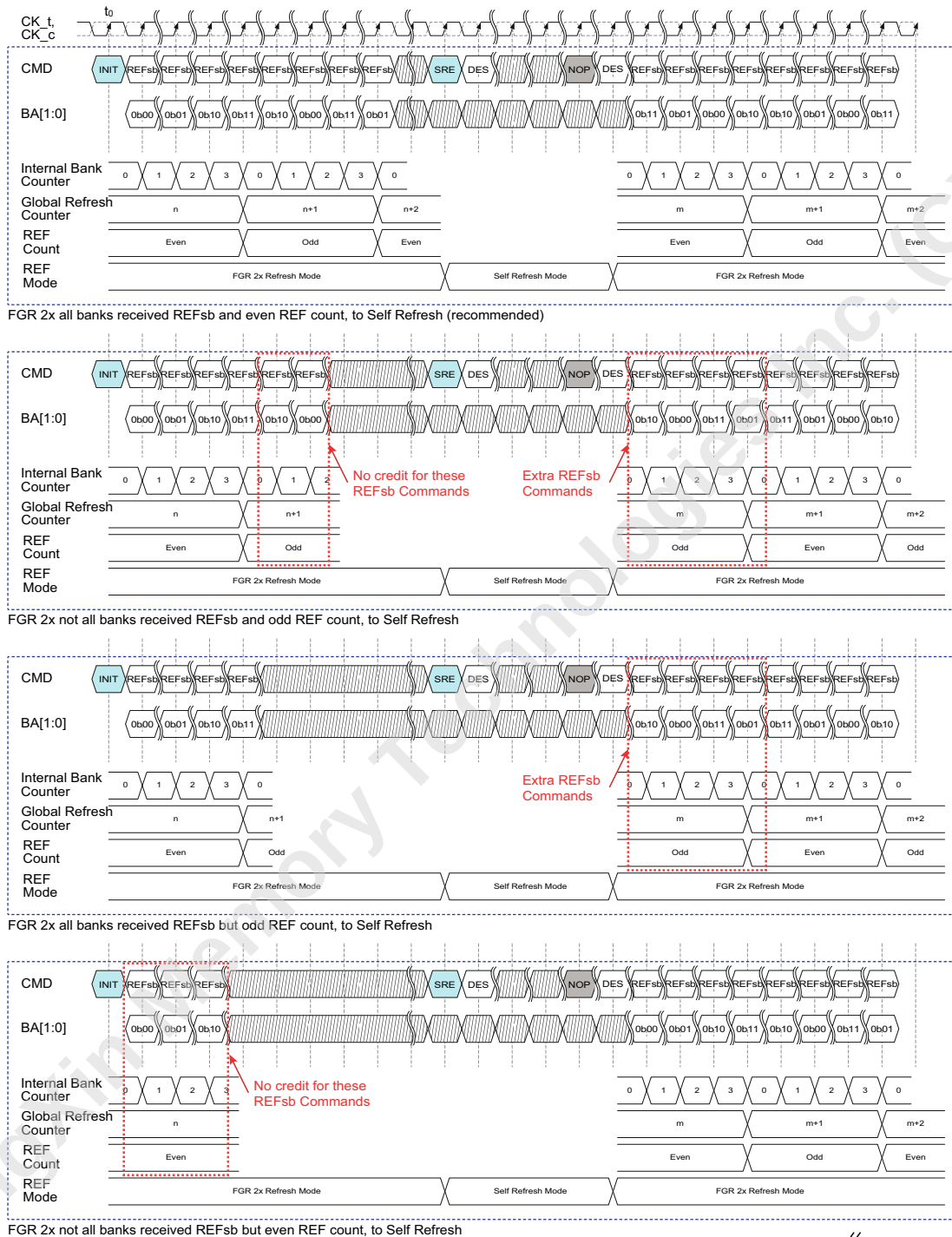
Figure 72 — 16 Gb and Higher Density DRAM FGR 2x REFsb to SREF Command Timing
