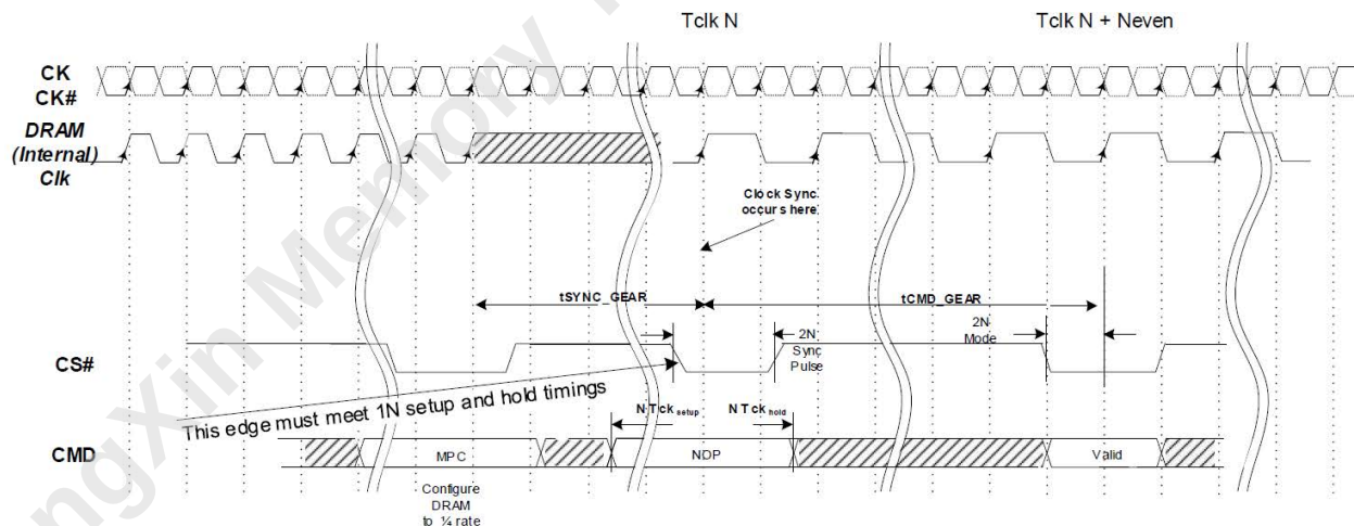
Figure 182 — Geardown During Initializations
