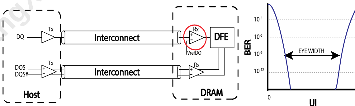
Figure 225 — Example of DDR5 Memory Interconnect
