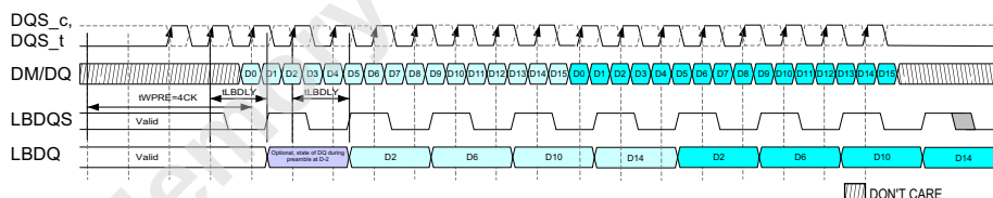
Figure 175 — Loopback Write Burst Output Mode 4-Way PhaseC Data Burst Bit and PhaseA Strobe Alignment WPRE=4CK Optional Example
