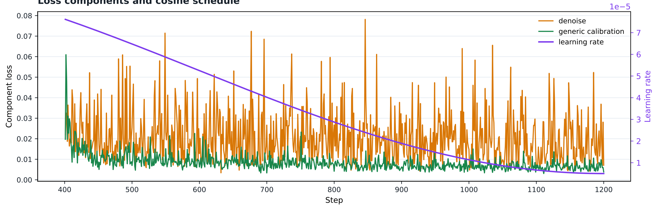
Loss components and cosine schedule
