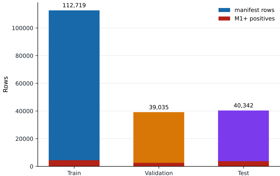
Frozen chronological partitions
