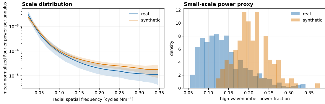
Figure 6.8: Fourier-space diagnostics for the observed and generated line-of-sight fields, including spectral centroid, high-wavenumber power fraction, and the normalized half-space potential proxy.
