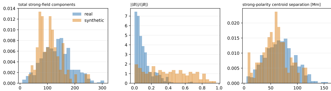
Figure 6.9: Strong-field connected-component counts and polarity-centroid separation for the real and generated fields.
