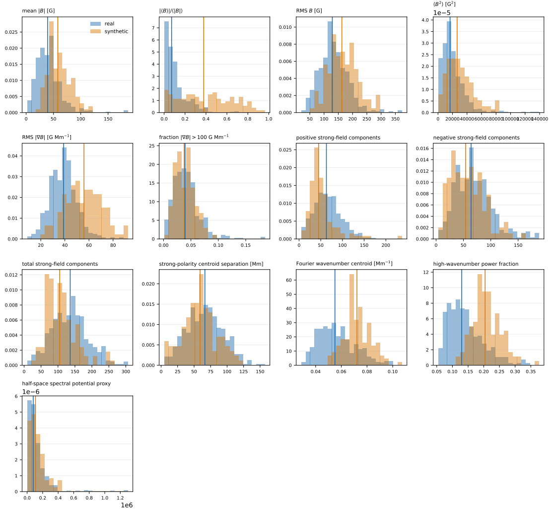
Figure 6.7: Independent line-of-sight proxy distributions for the real positive audit set and the generated BASE set. These scalar diagnostics are descriptive and are not a 3D coronal-field evaluation.
