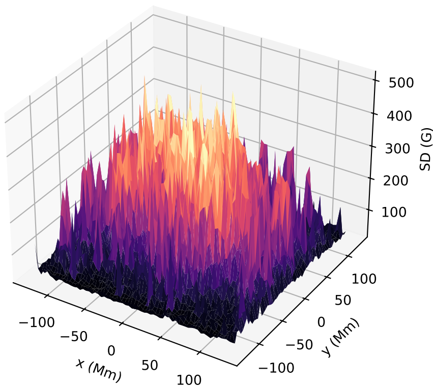
Spread as a surface
