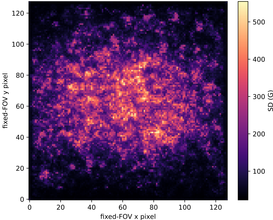
Pixelwise ensemble spread
