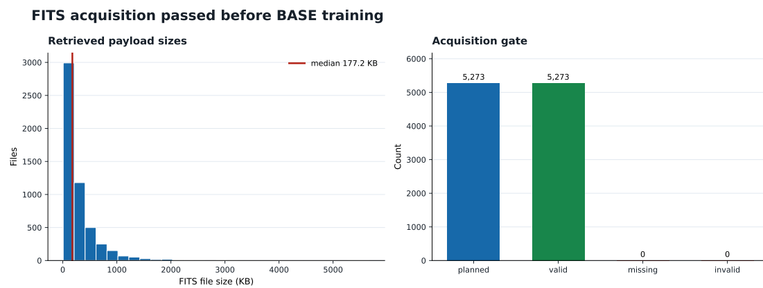
Figure 3.3: FITS acquisition accounting and the distribution of local payload sizes. The right-hand panel is the gate that unlocked the model stage.
