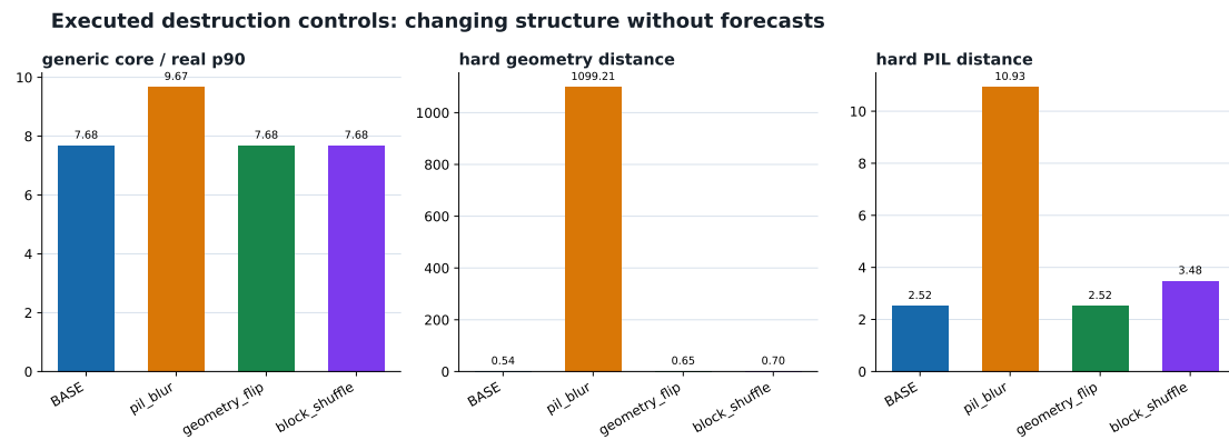
Figure 10.3: Executed counterfactual destruction controls. The panels report independent distances after transforming the generated fields; no forecasting output is involved.
