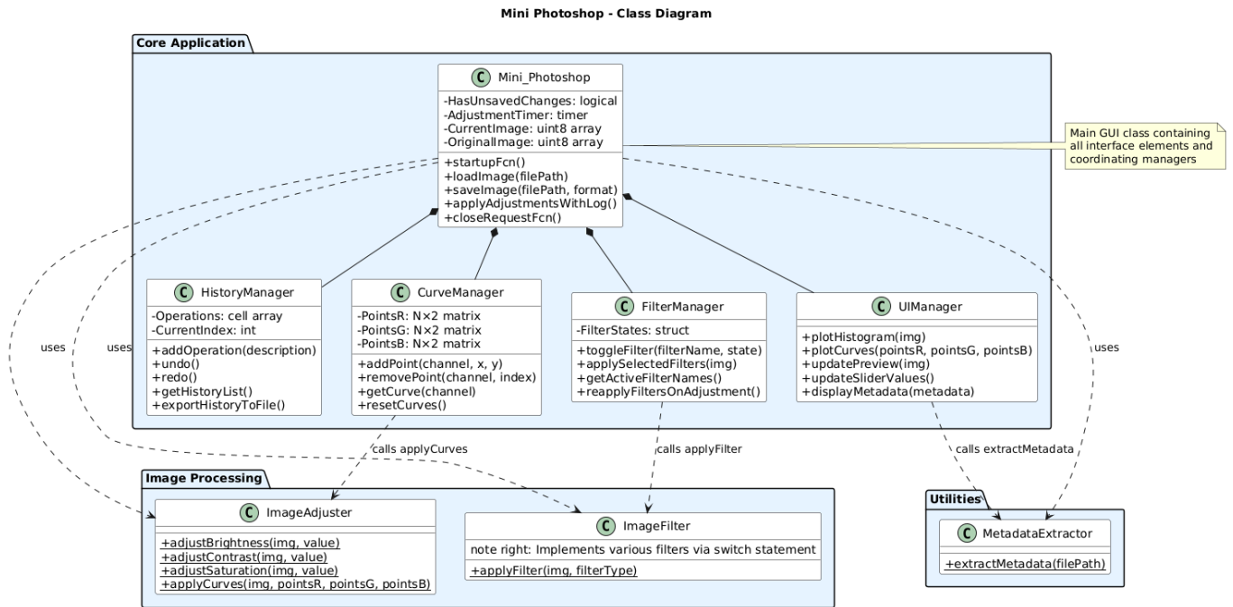
Fig. 1. UML Class Diagram showing the modular architecture of Mini Photoshop
