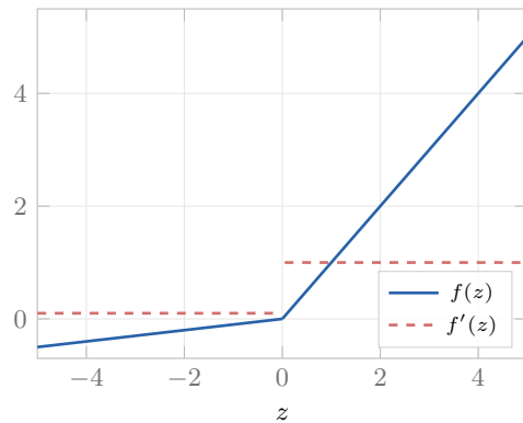
Leaky ReLU ( \alpha = 0,1 )
