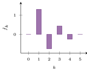
Coefficientes \hat{f}_k = U^\top f
