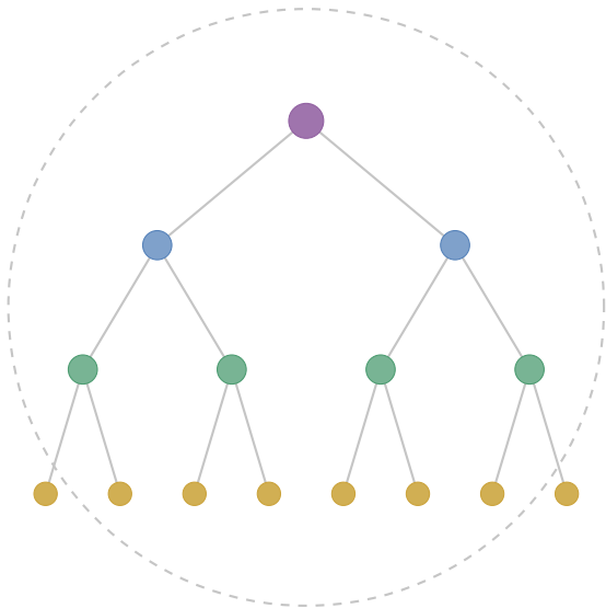
Embedding euclidiano
