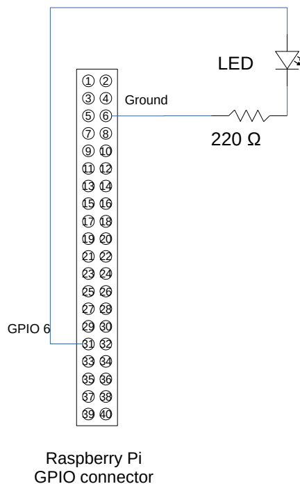
Figure 2. Schematic circuit of LED connected to the Raspberry Pi GPIO.
