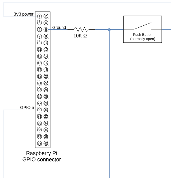
Figure 2. Schematic diagram of the push button circuit connected to the Raspberry Pi GPIO.
