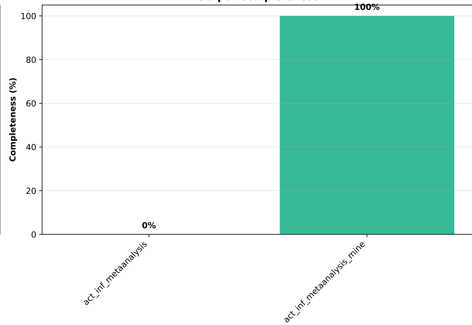
Output Completeness
