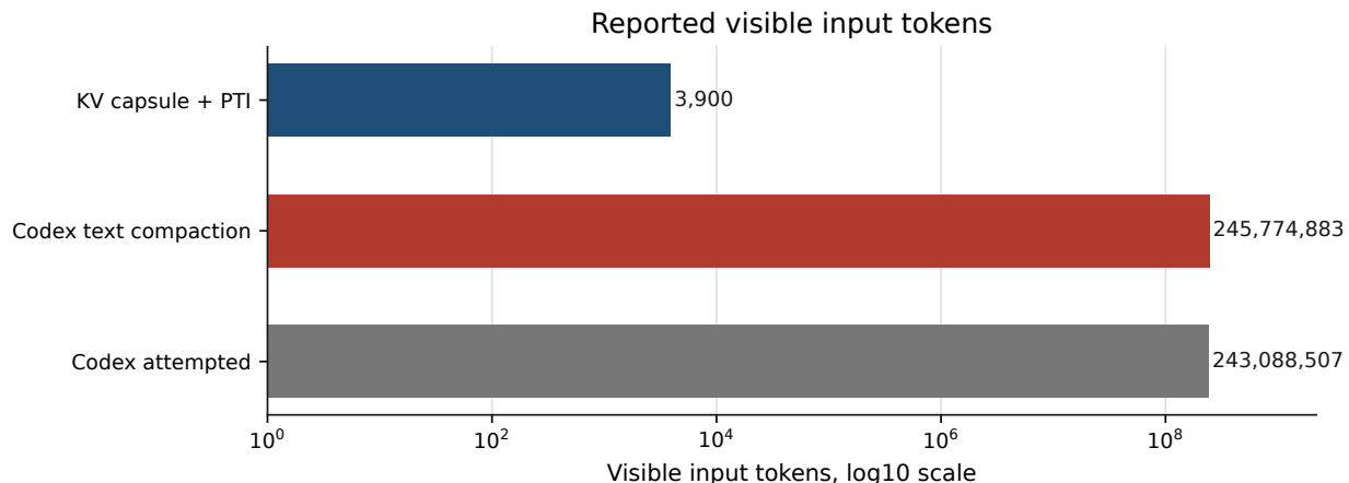
Figure 2: Repeated-work visible input burden. Log scale is used because the runtime gap is several orders of magnitude. The baseline telemetry is cumulative reported burden, not clean per-task token accounting.
