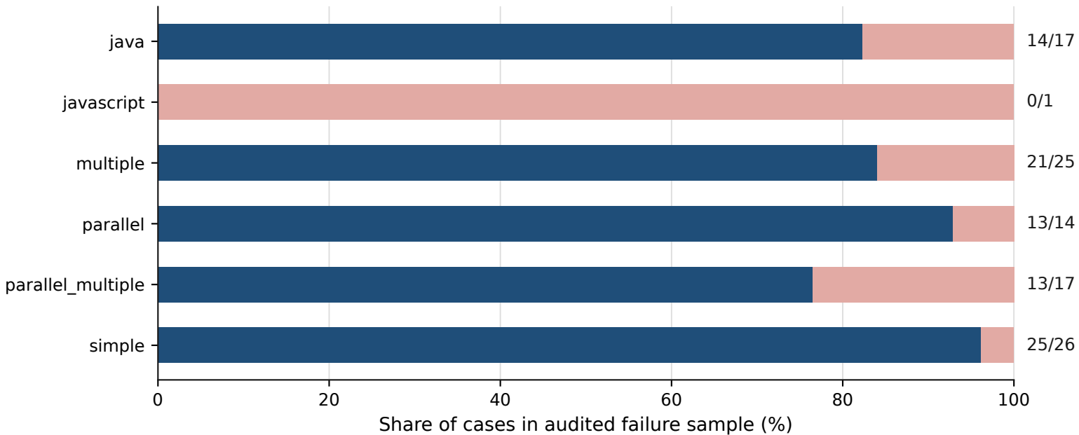
Natural Codex/Ollama pass/fail by BFCL category
