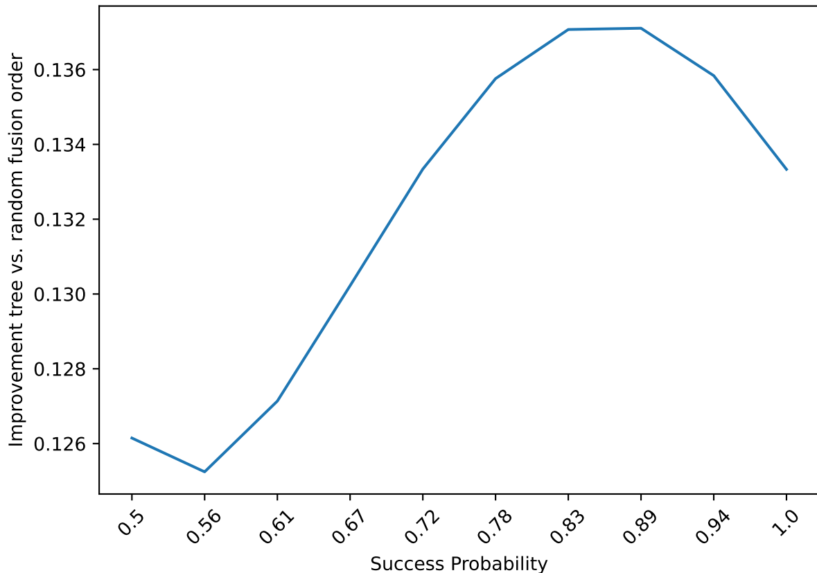
Avg. FP times percentage for tree vs. random fusion order (n=5)
