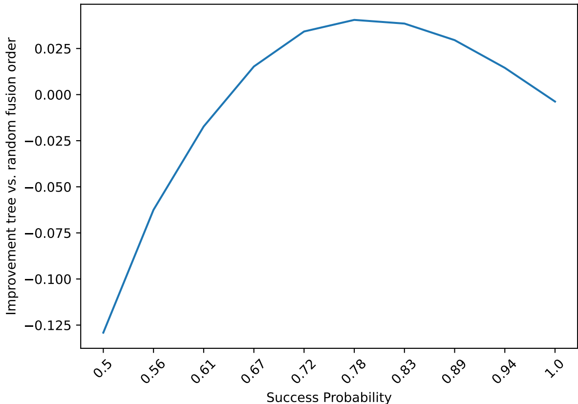
Avg. FP times percentage for tree vs. random fusion order (n=9)
