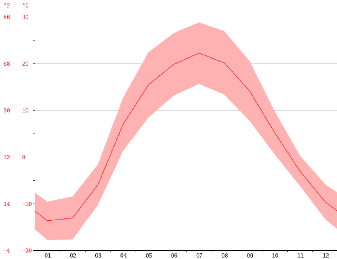
Figure 16: Graph of the real average temperatures in Orenburg during one year (source: https://it.climate-data.org/location/475/#temperature-graph ).
