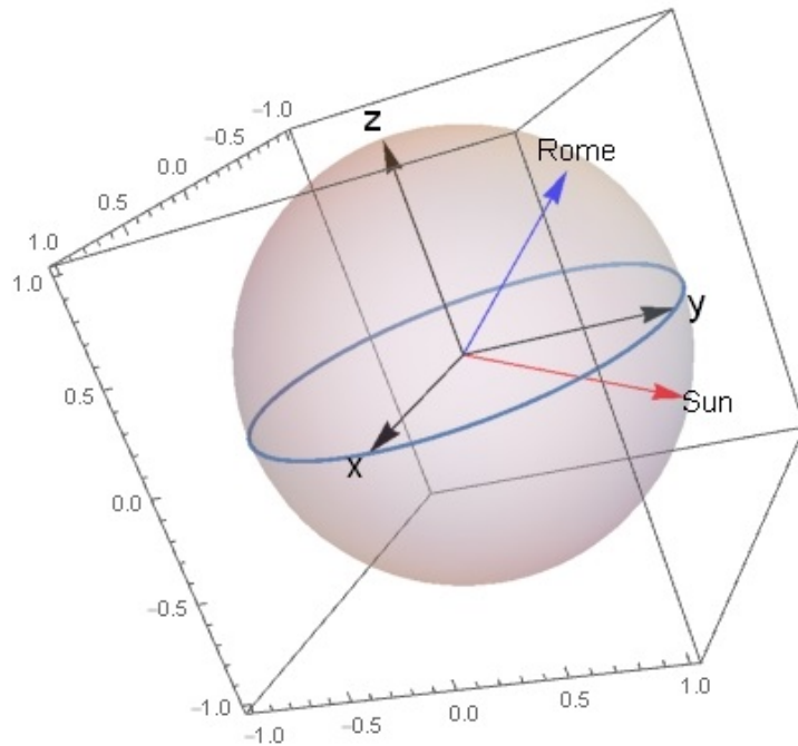
Figure 6: Cartesian reference system on the Earth. In the graph there is also a vector in red that indicates the solar ray and a vector in blue pointing to Rome at midday on the winter solstice.
