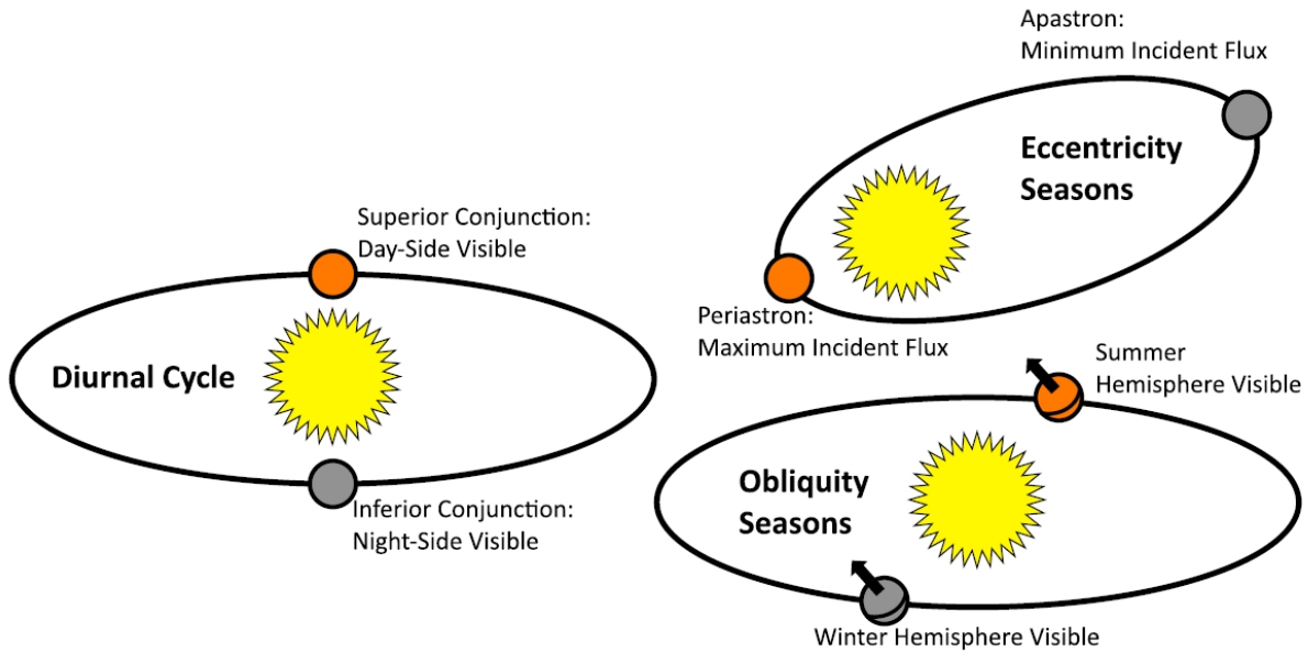
Figure 1: Sources of Thermal phase variations. Redrawn after Cowan, Voigt and Abbot [7].
