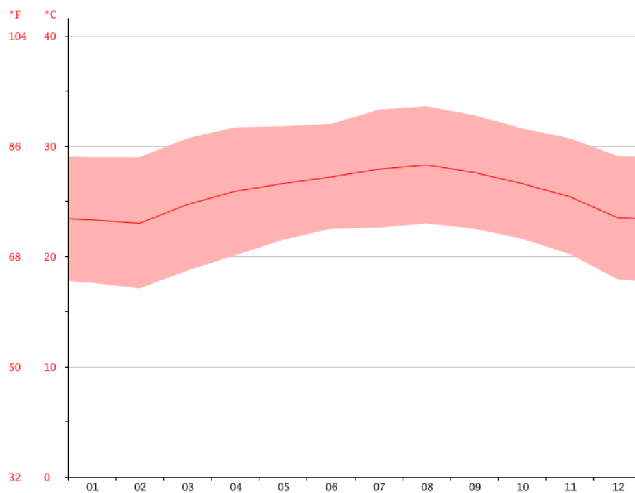
Figure 14: Graph of the real average temperatures in Haiti during one year (source: https://it.climate-data.org/location/687081/#temperature-graph ).
