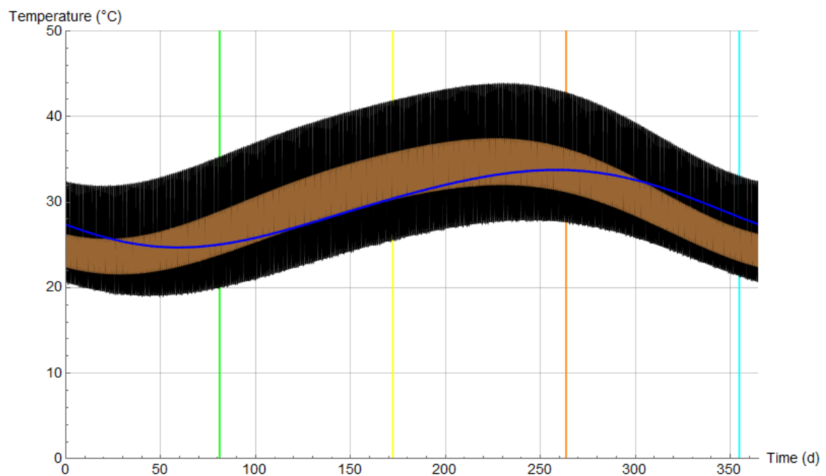
Figure 13: Thermal phase variations during one year in Haiti according to the 2ILCM.
