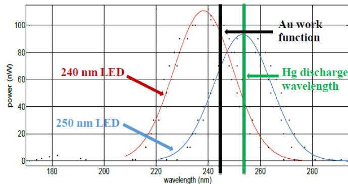
Figure 5: Gaussian fit to measurements of the UV-LEDs' intensity spectrum compared with the work function of Au and the Hg lamp discharge wavelength [4].
