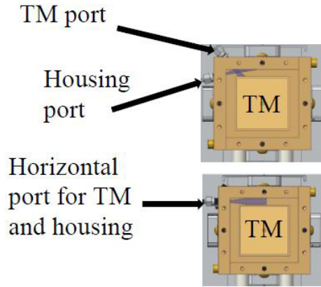
Figure 4: UV light ports design [4]
