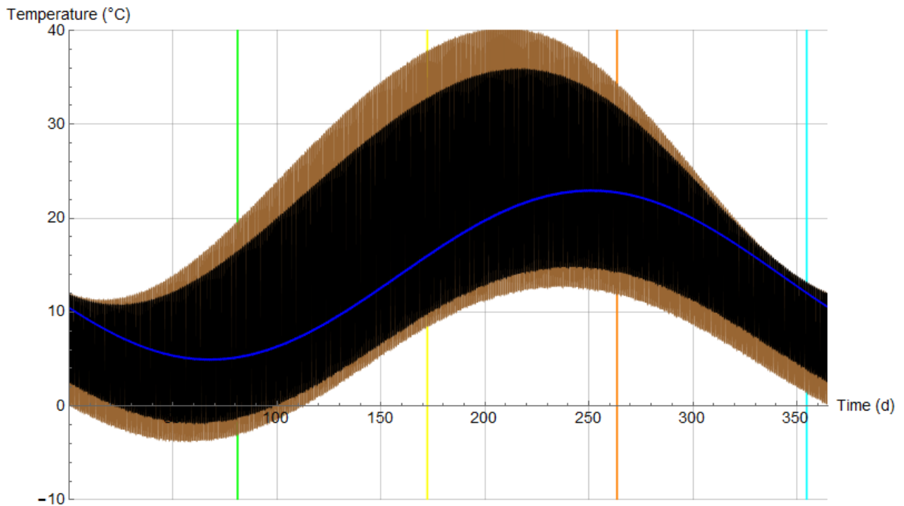
Figure 17: Thermal phase variations during one year in Rome with sand instead of ground according to the 2ILCM.
