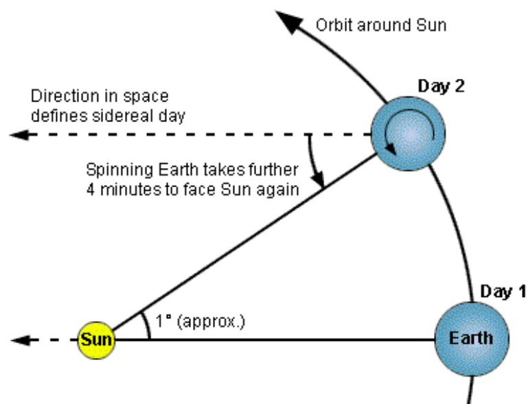
Figure 4: The solar day is longer than the sidereal day of around 4 minutes (source: https://hamptonphysics.wikispaces.com/sidereal+day ).
