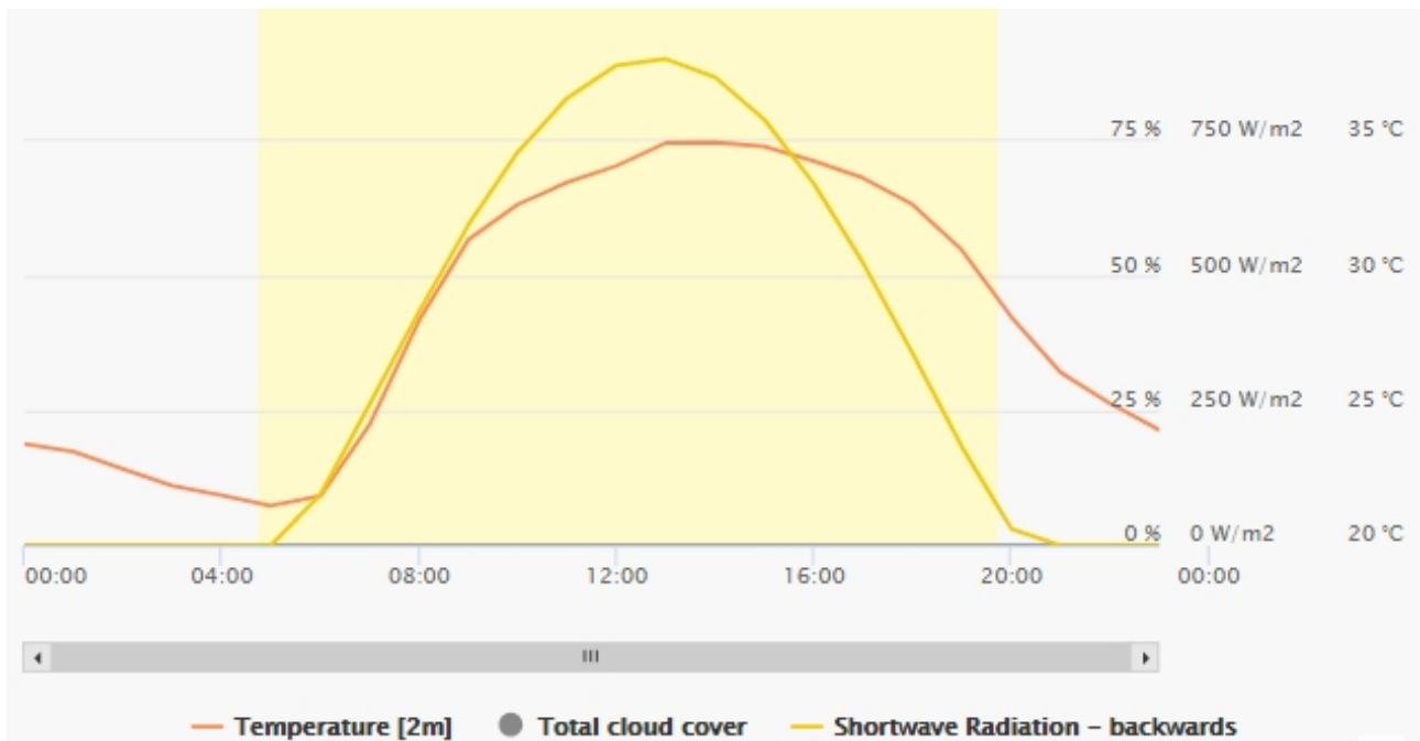
Figure 10: Real temperature in Rome on the 9th of July (2017) (source: https://www.meteoblue.com/ ).
