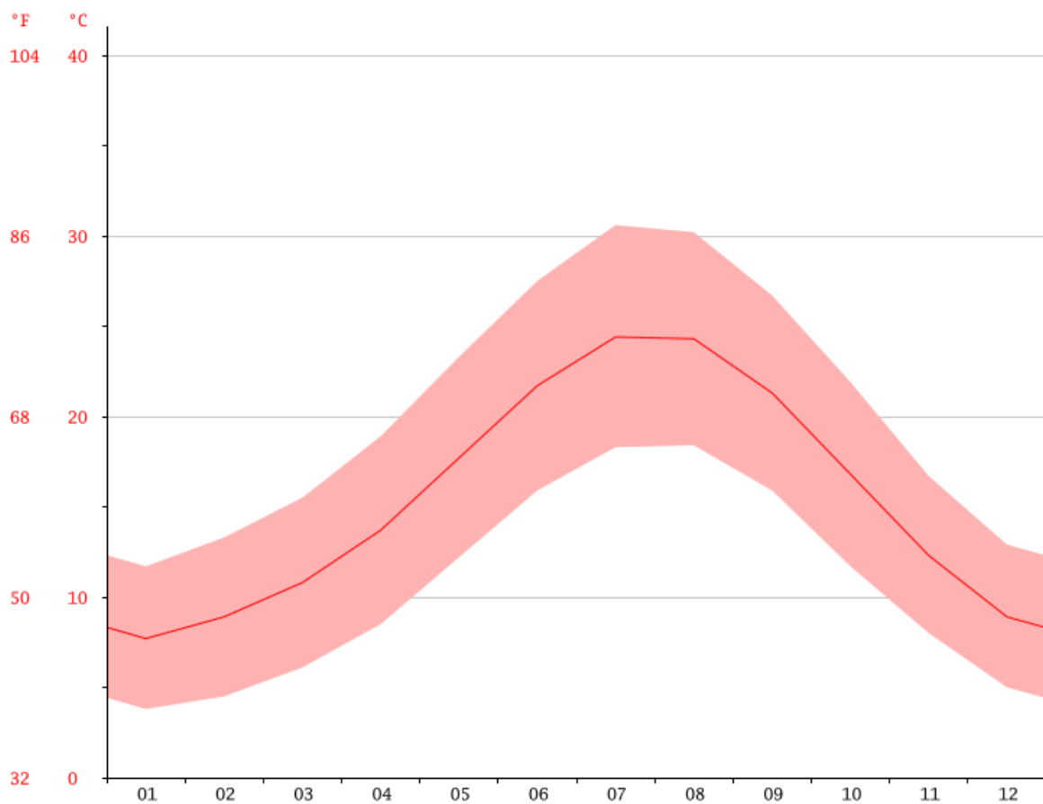
Figure 9: Graph of the real average temperatures in Rome during one year (source: https://it.climate-data.org/location/1185/#temperature-graph ).
