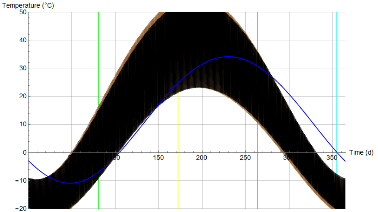
Figure 18: Thermal phase variations during one year in Rome with 90% of sand according to the 2ILCM.
