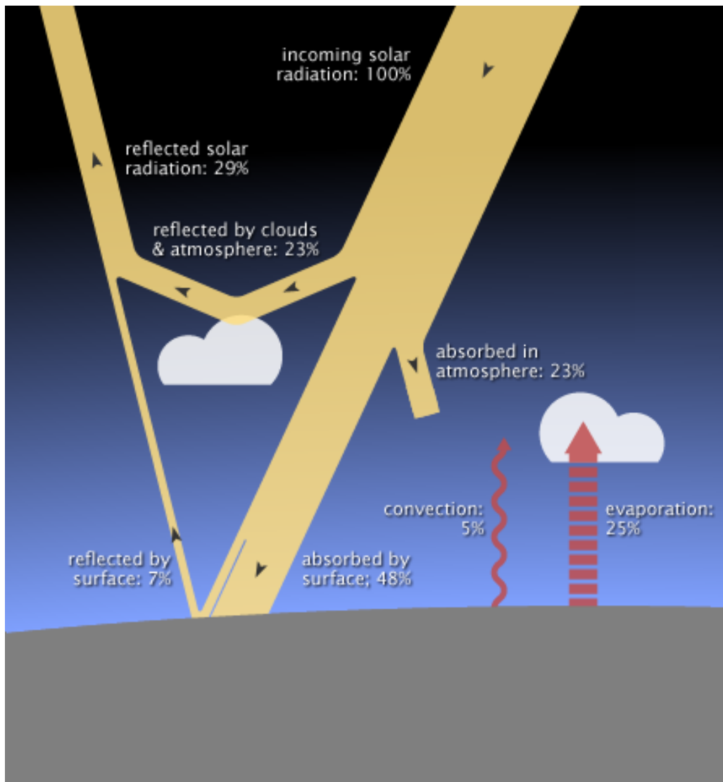
Figure 5: Global energy budget components (taken from NASA illustration by Robert Simmon, adapted from Trenberth, Fasullo and Kiehl [27], using CERES flux estimates provided by Norman Loeb).
