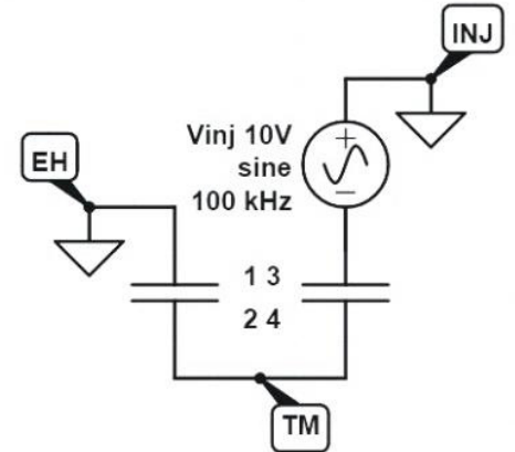
Figure 3: Circuit model for AC charge control
