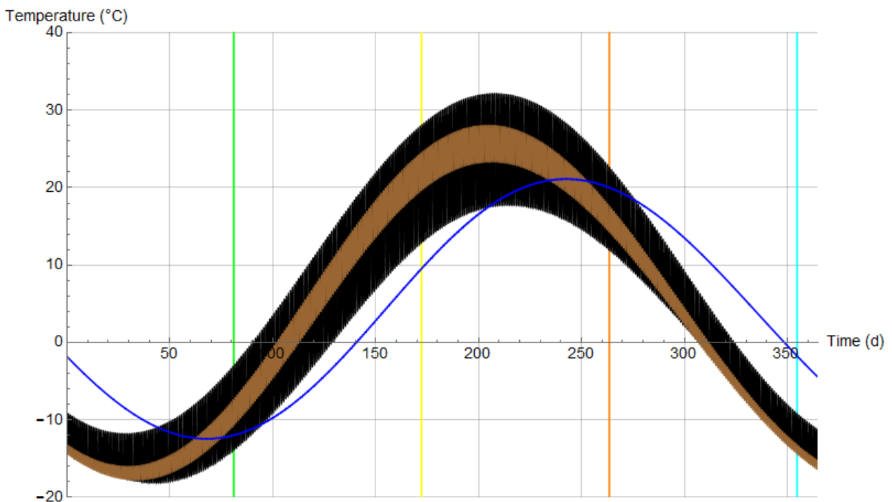
Figure 15: Thermal phase variations during one year in Orenburg with 80% of ground according to the 2ILCM.
