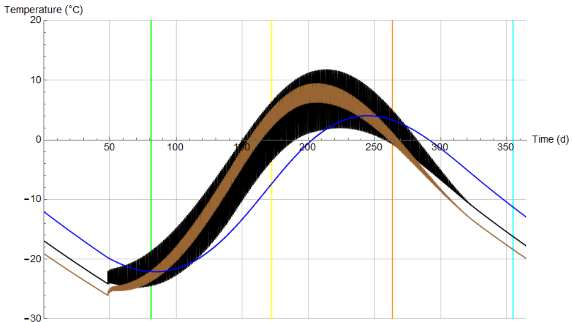
Figure 11: Thermal phase variations during one year in Finnmark according to the 2ILCM.
