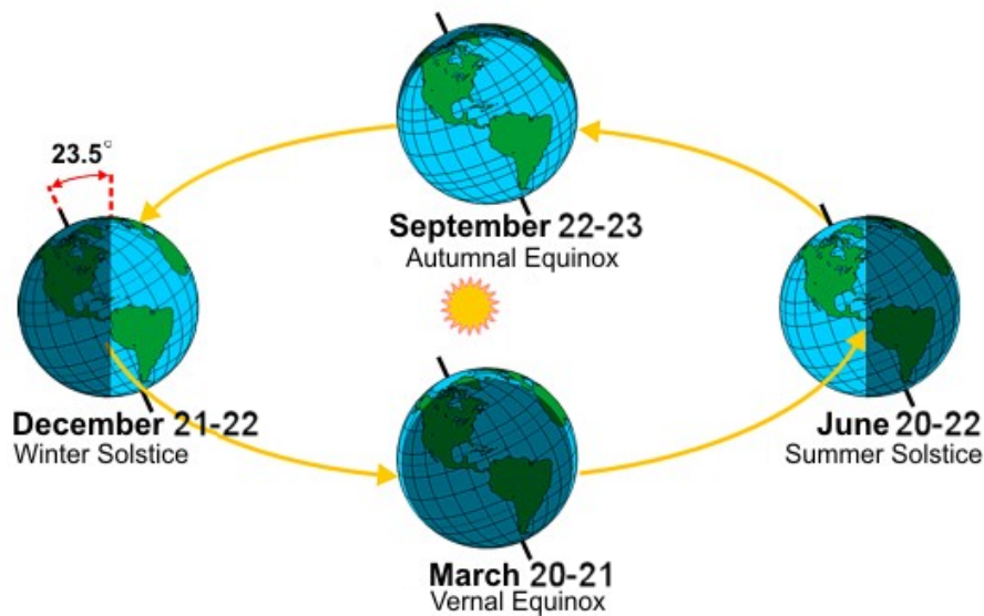
Figure 3: Revolution motion of the earth around the Sun.
