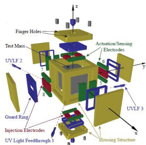
Figure 1: Exploded view of the LISA Pathfinder inertial sensor including the cubical test mass, the electrode housing structure with the actuation/sensing, and injection electrodes. [2]
