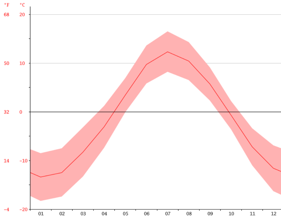
Figure 12: Graph of the real average temperatures in Finnmark during one year (source: https://it.climate-data.org/location/19645/#temperature-graph ).
