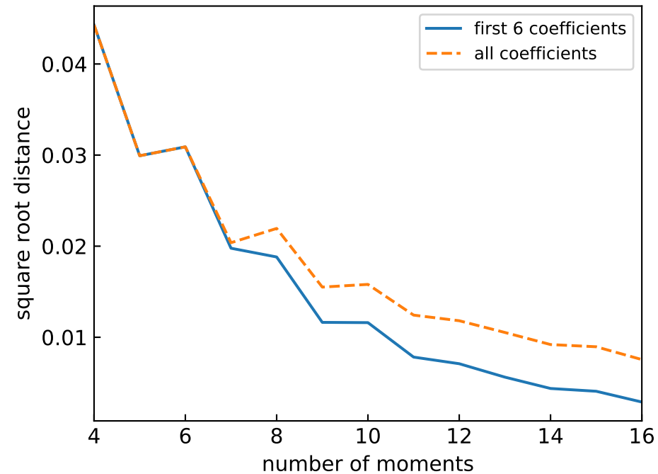
Hermite polynomials
