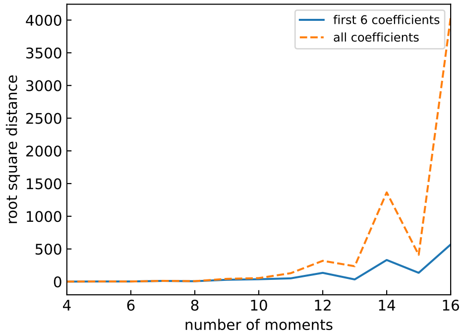
Logistic polynomials
