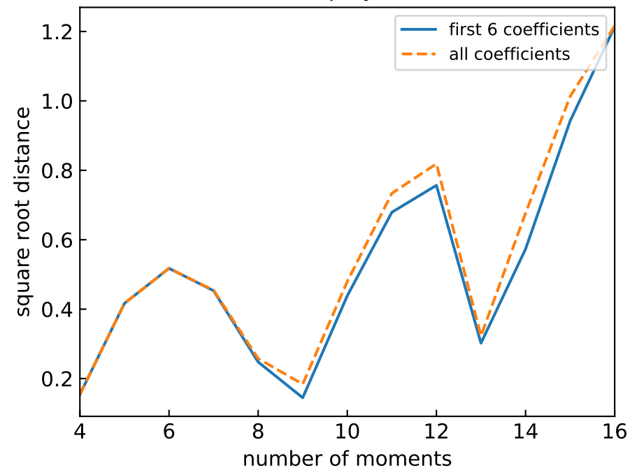
Hermite polynomials
