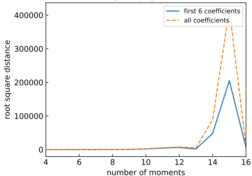
Logistic polynomials
