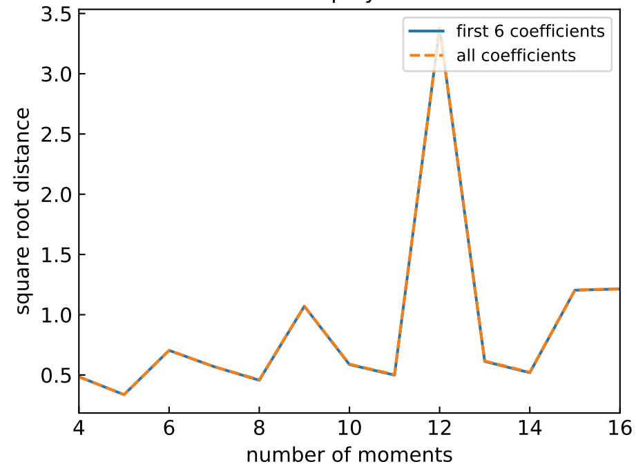
Hermite polynomials
