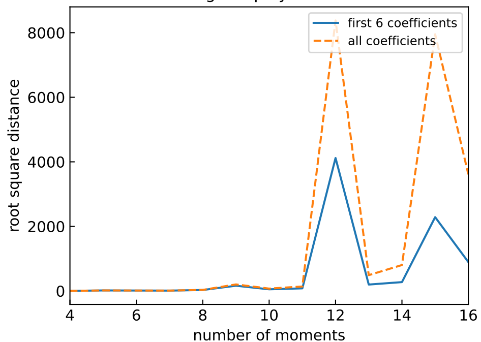
Logistic polynomials
