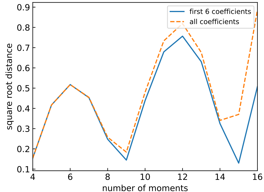
Hermite polynomials
