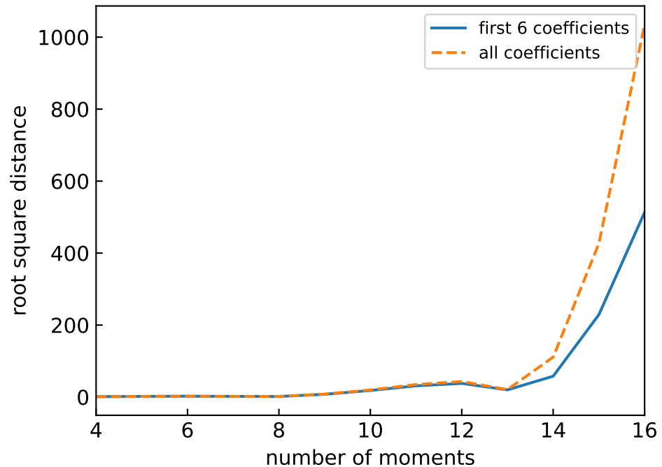
Logistic polynomials
